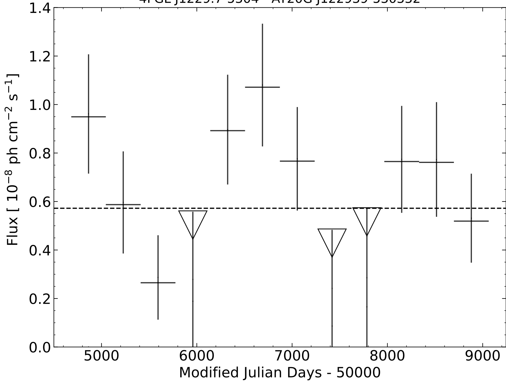
4FGL J1229.7-5304 - AT20G J122939-530332
