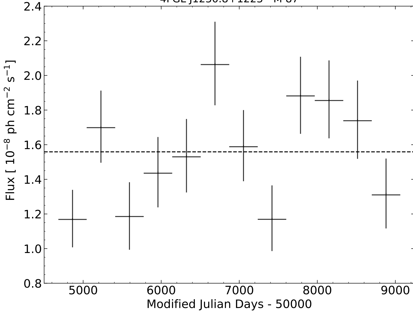
4FGL J1230.8+1223 - M 87
