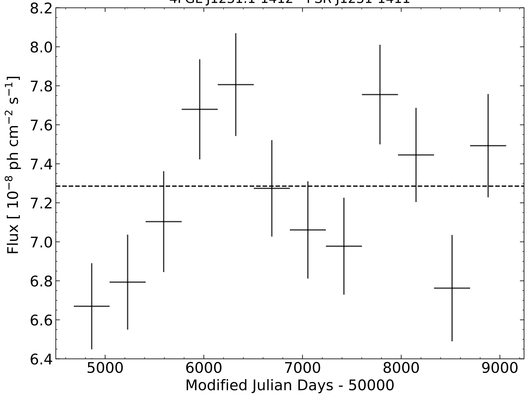
4FGL J1231.1-1412 - PSR J1231-1411
