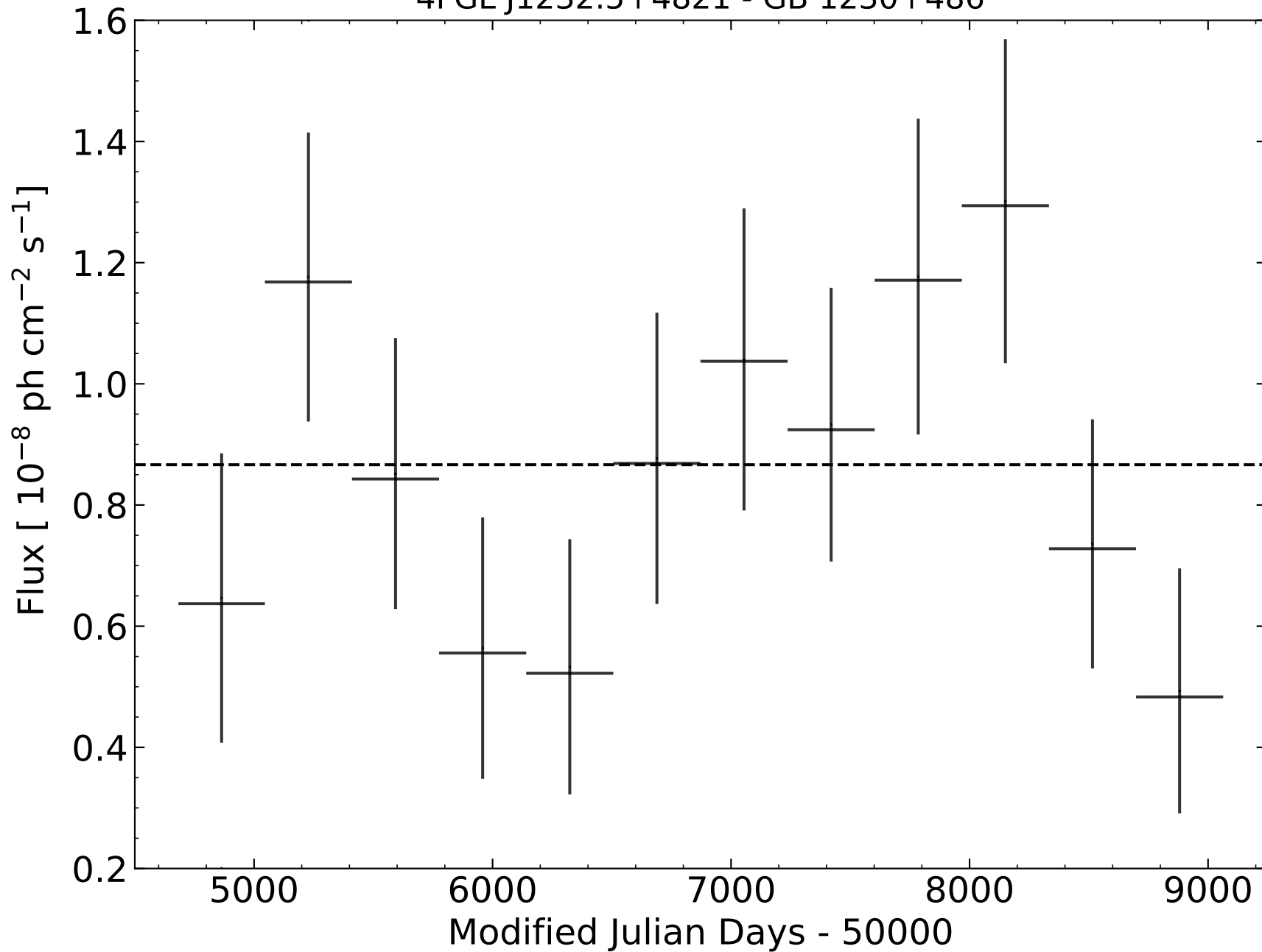
4FGL J1232.5+4821 - GB 1230+486
