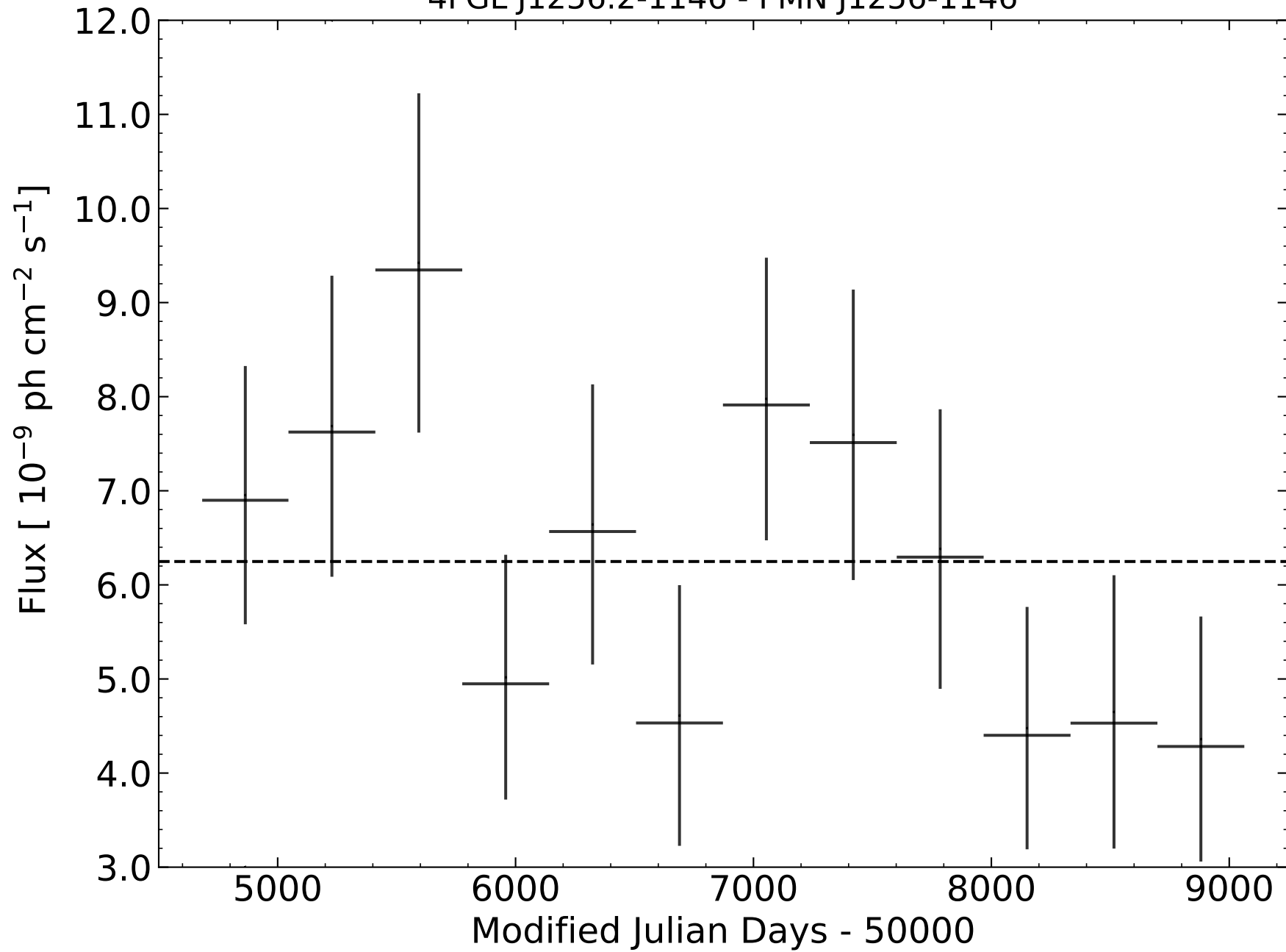
4FGL J1256.2-1146 - PMN J1256-1146
