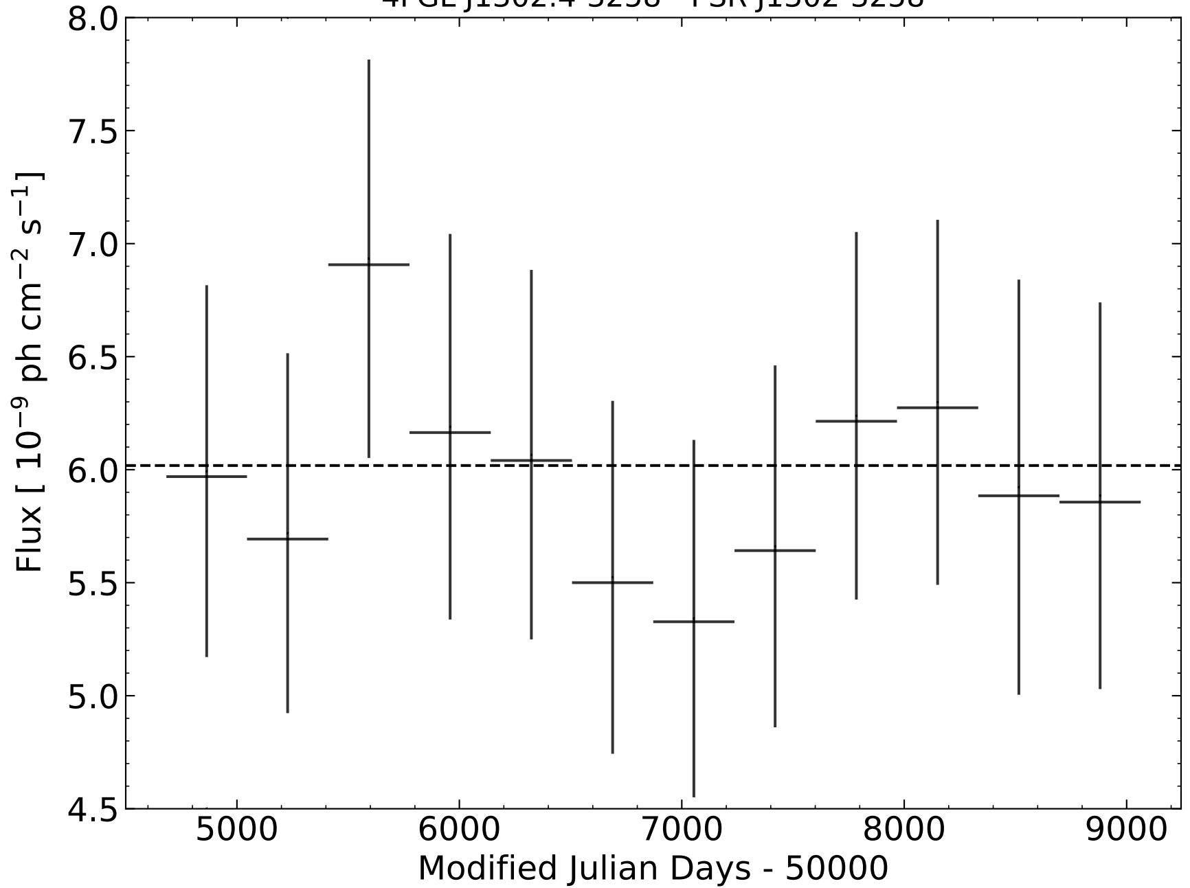
4FGL J1302.4-3258 - PSR J1302-3258
