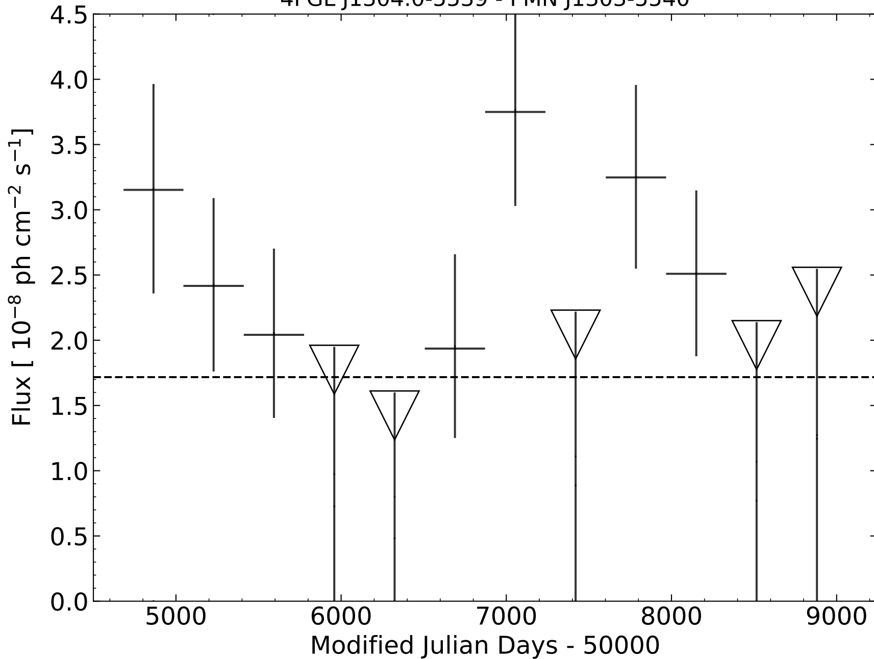
4FGL J1304.0-5539 - PMN J1303-5540
