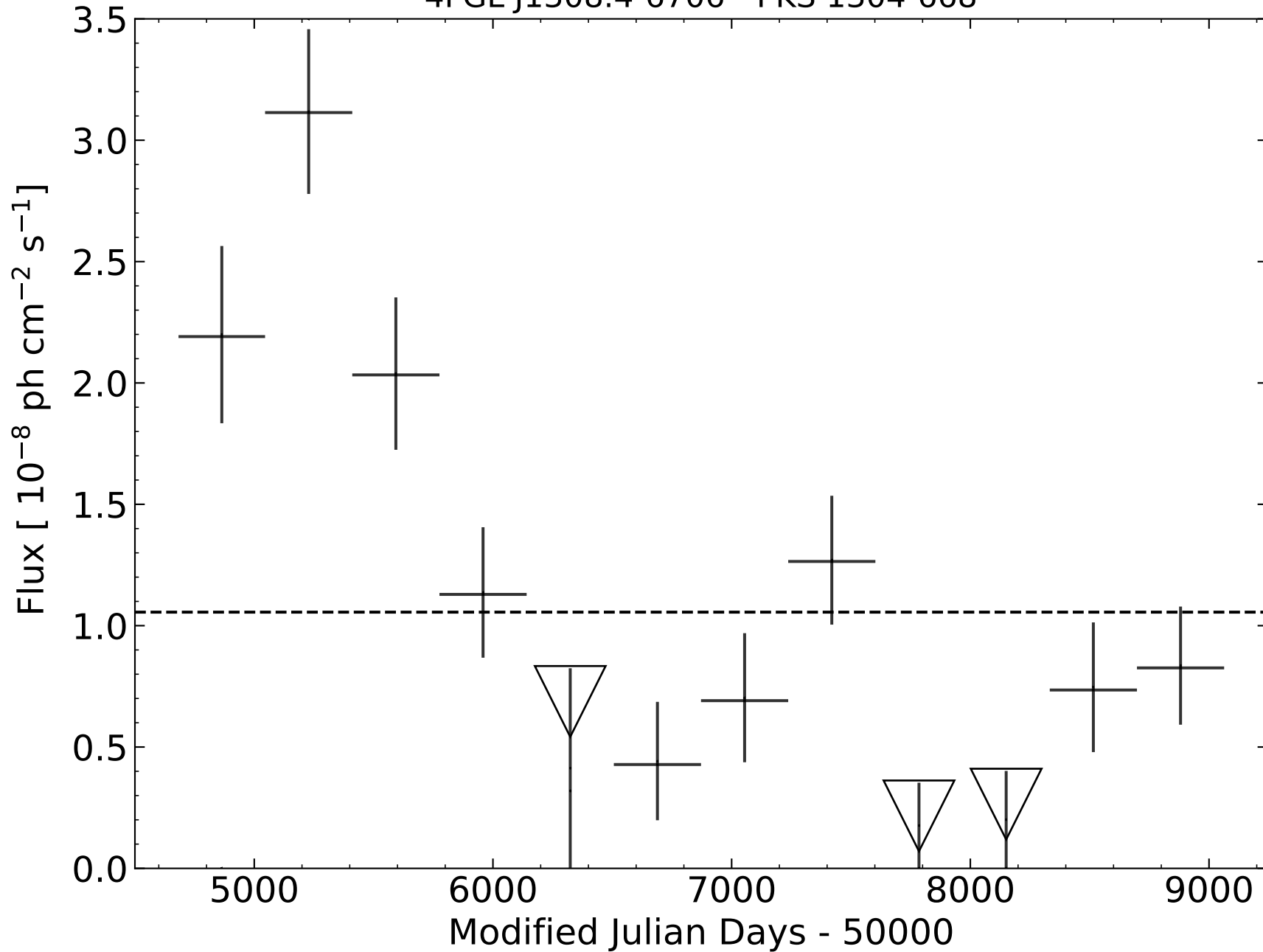
4FGL J1308.4-6706 - PKS 1304-668
