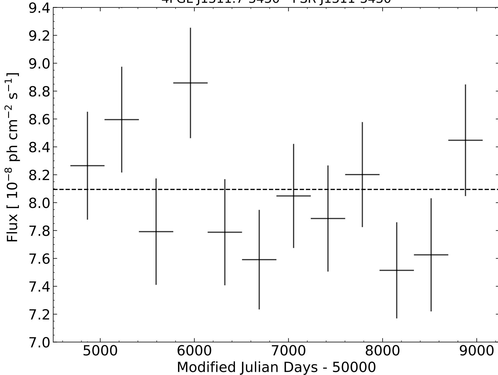
4FGL J1311.7-3430 - PSR J1311-3430
