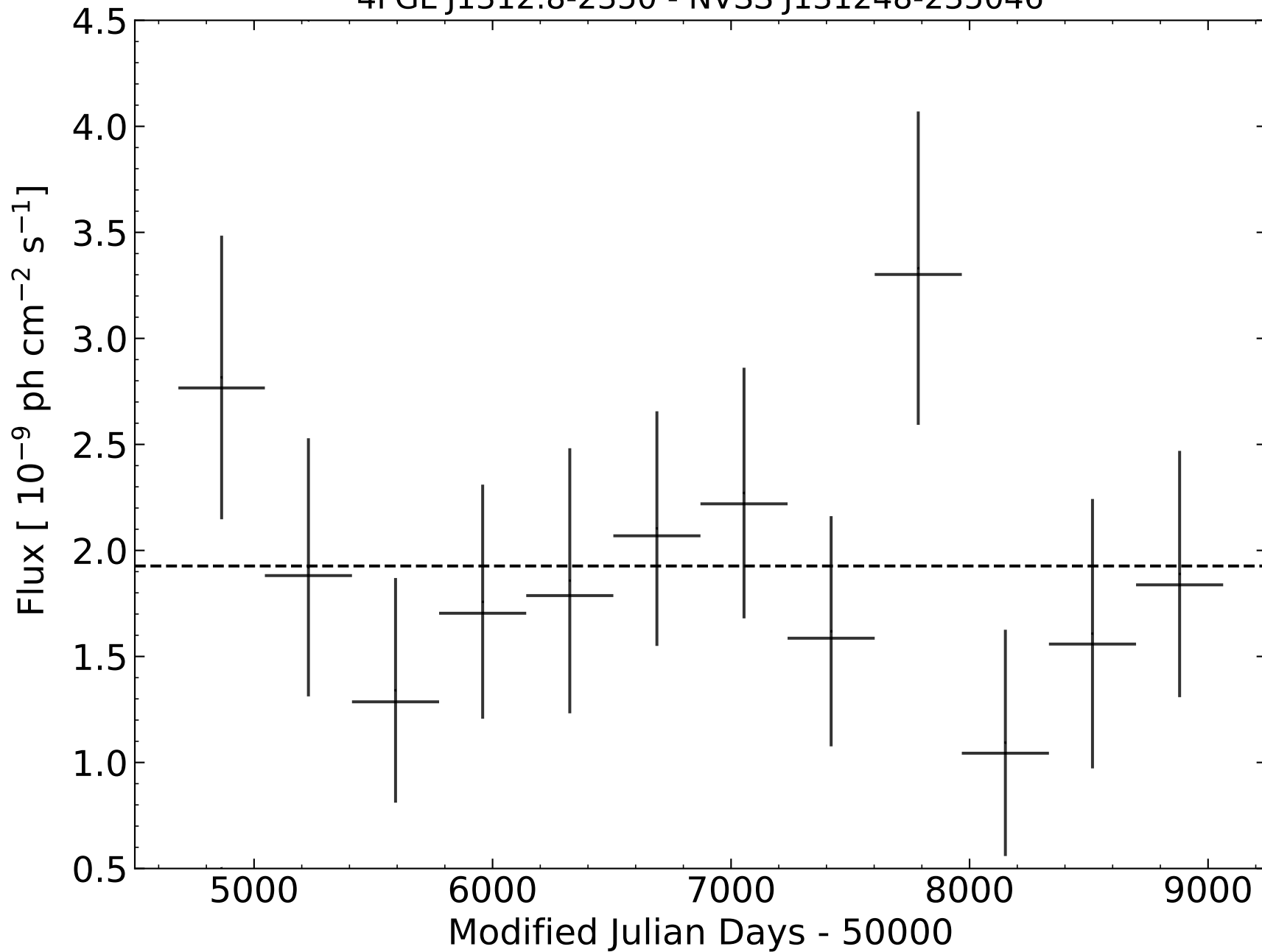
4FGL J1312.8-2350 - NVSS J131248-235046
