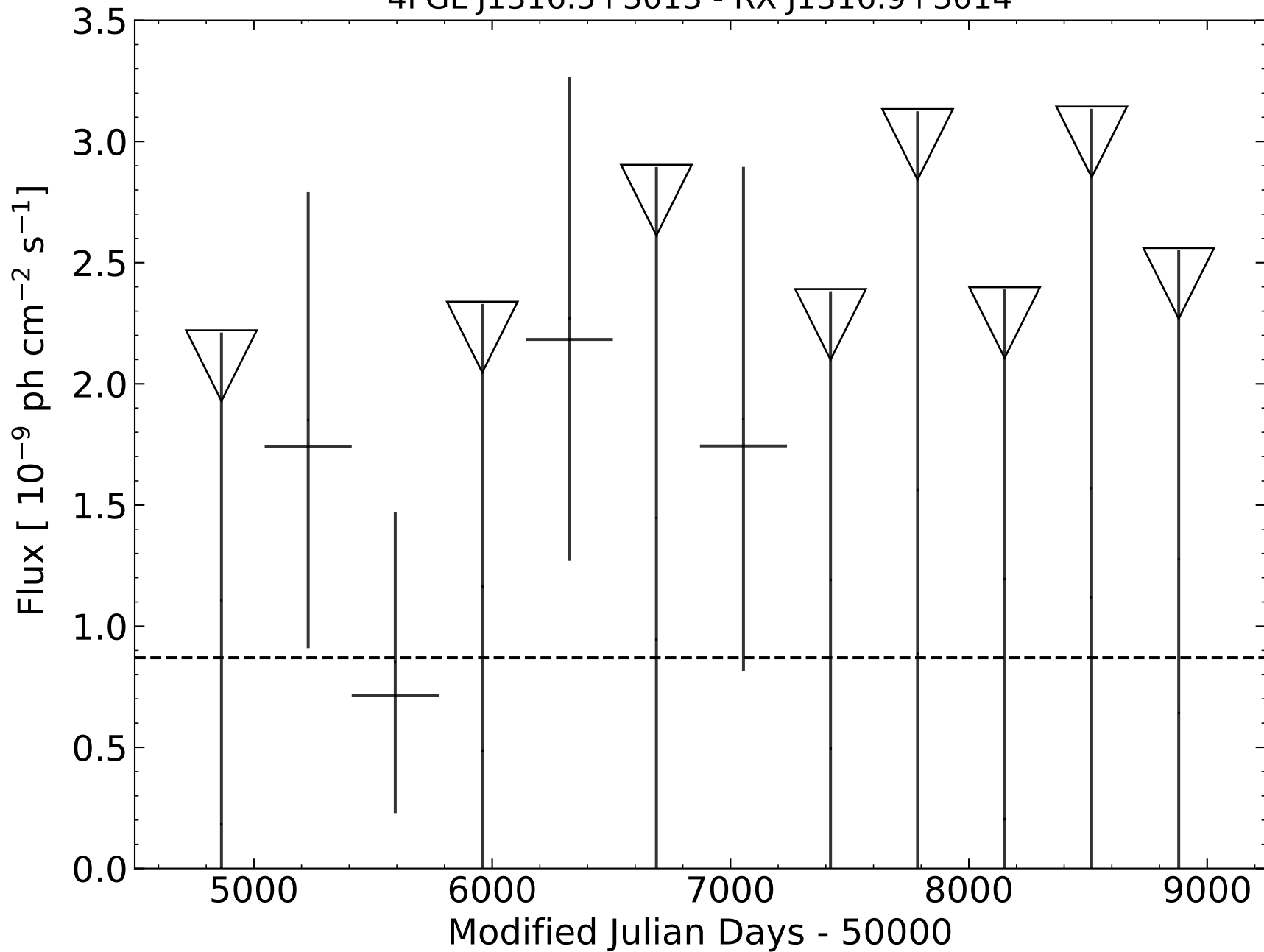
4FGL J1316.5+3013 - RX J1316.9+3014
