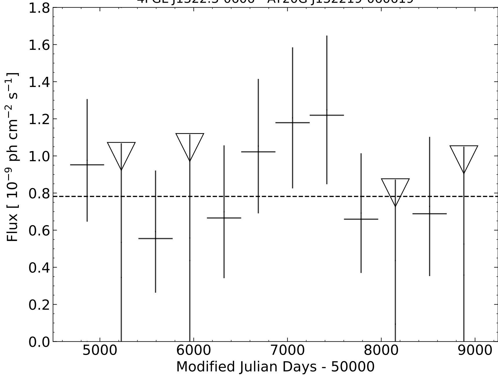
4FGL J1322.3-0606 - AT20G J132219-060619
