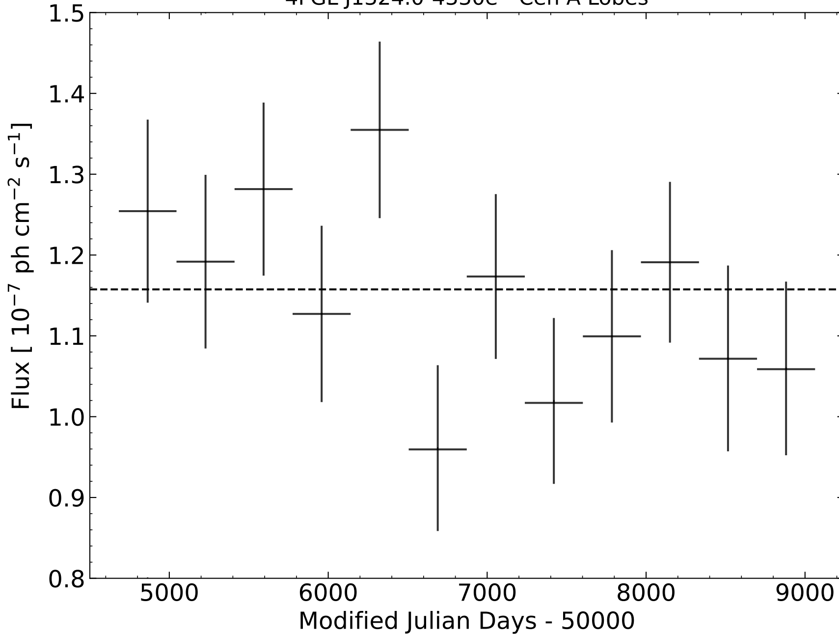
4FGL J1324.0-4330e - Cen A Lobes
