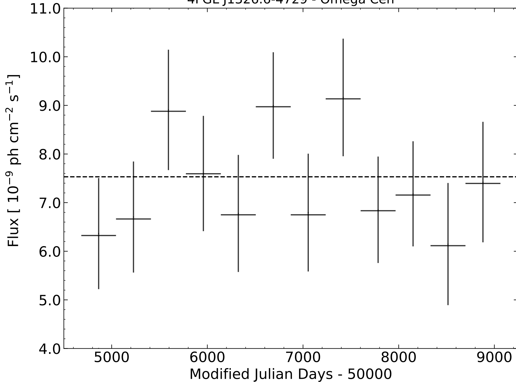
4FGL J1326.6-4729 - Omega Cen
