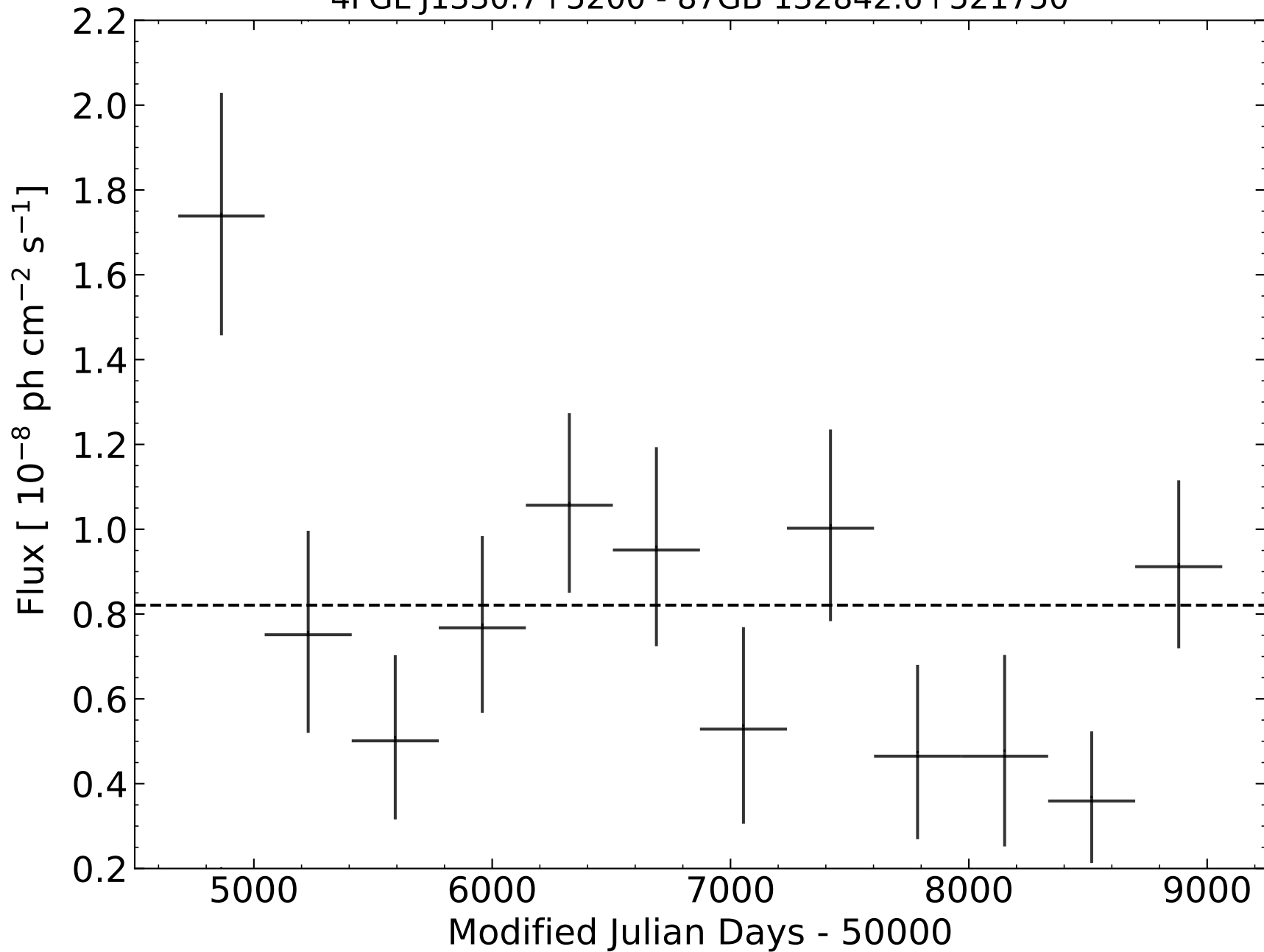
4FGL J1330.7+5200 - 87GB 132842.6+521750
