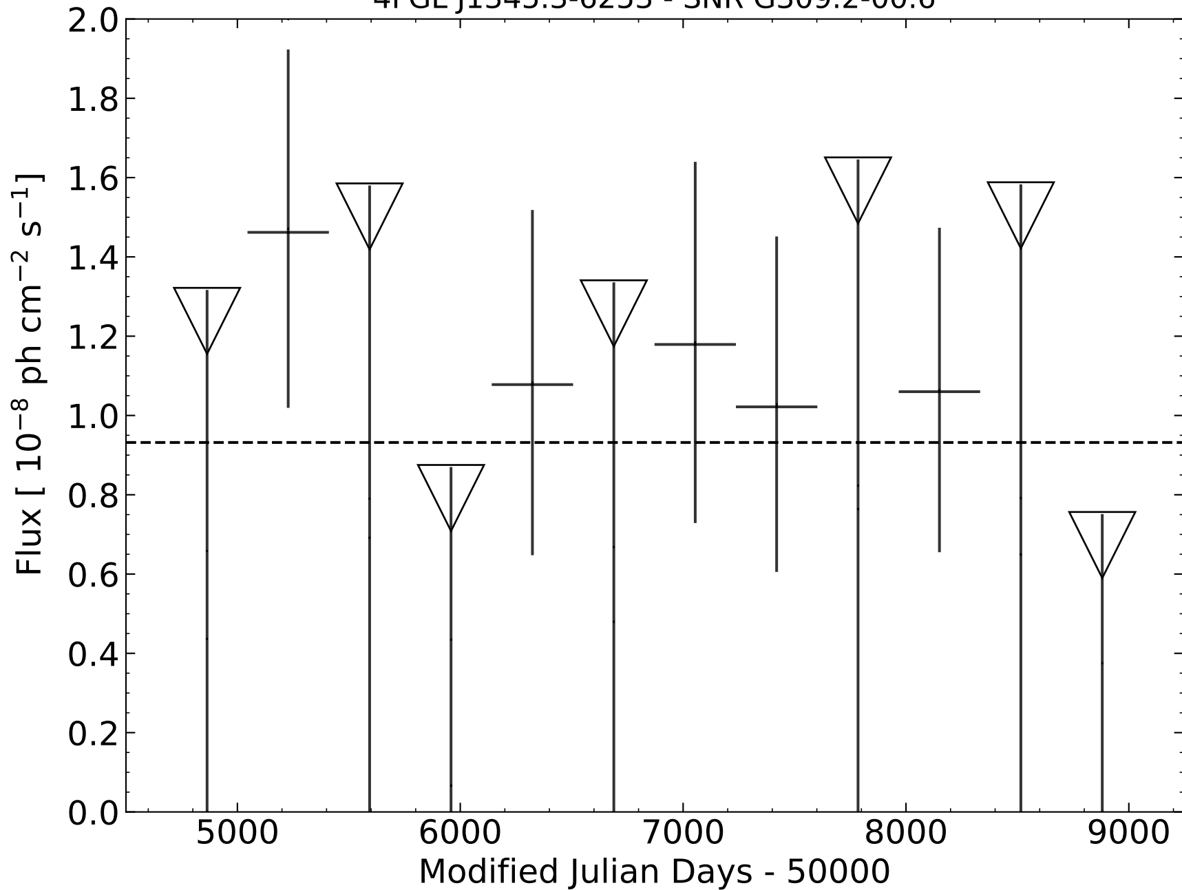
4FGL J1345.3-6253 - SNR G309.2-00.6
