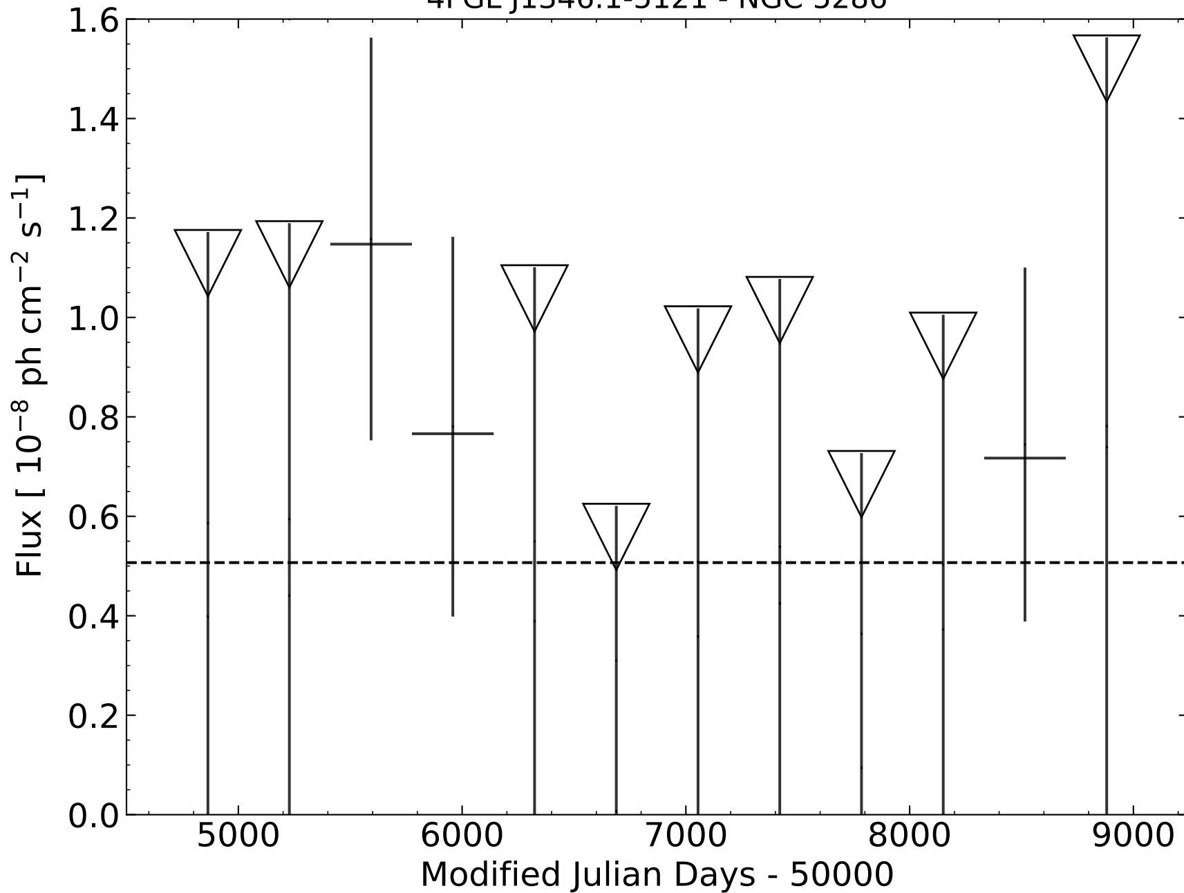
4FGL J1346.1-5121 - NGC 5286
