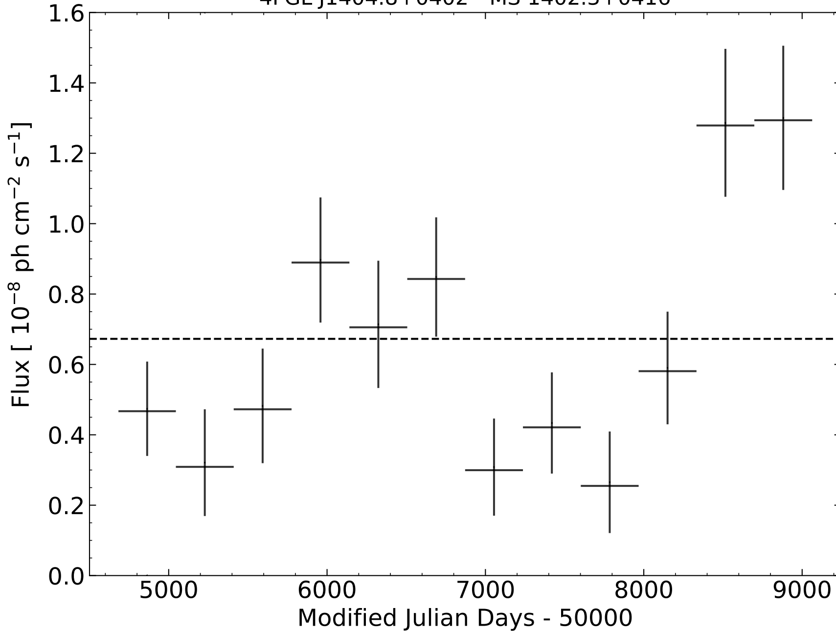
4FGL J1404.8+0402 - MS 1402.3+0416
