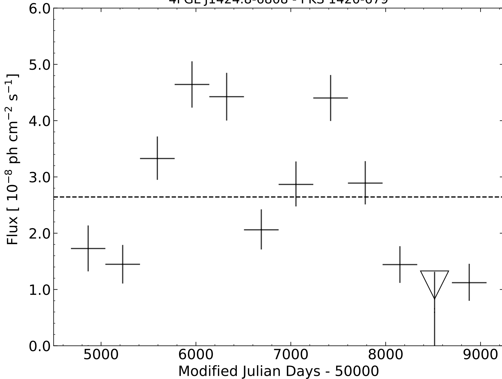
4FGL J1424.8-6808 - PKS 1420-679
