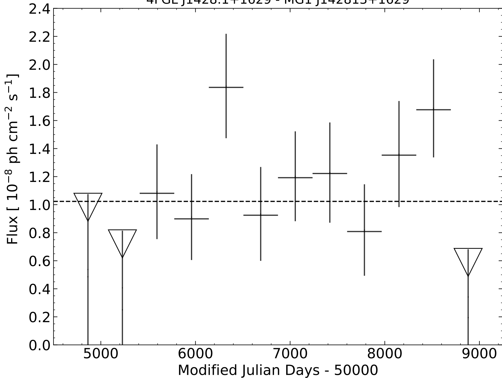
4FGL J1428.1+1629 - MG1 J142813+1629
