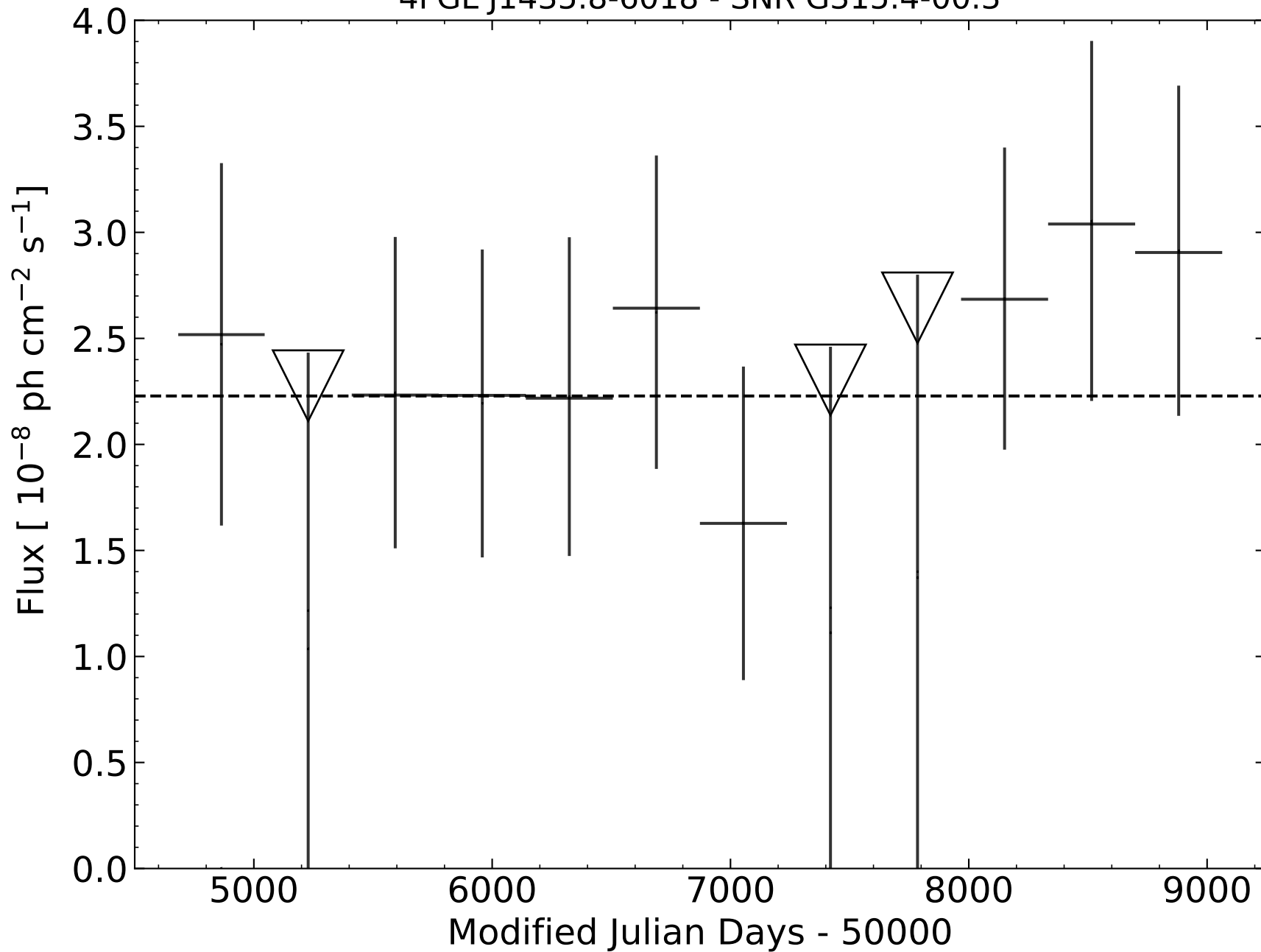
4FGL J1435.8-6018 - SNR G315.4-00.3
