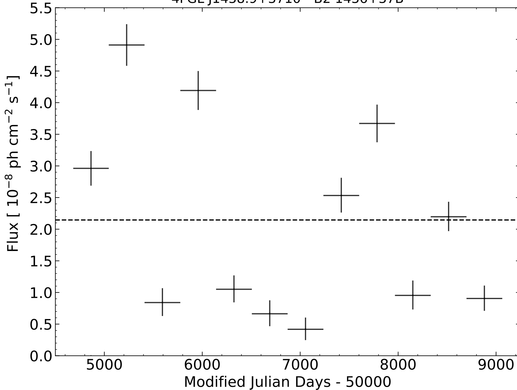
4FGL J1438.9+3710 - B2 1436+37B
