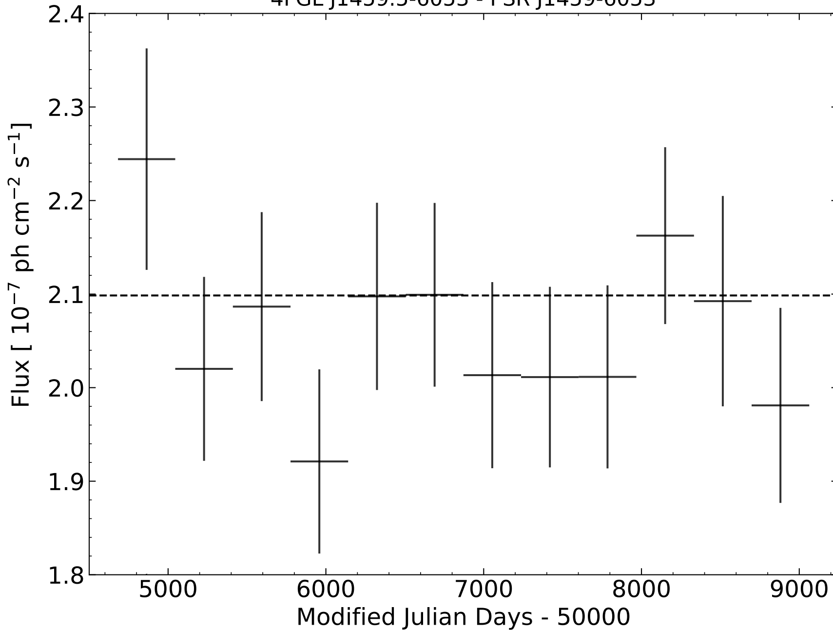
4FGL J1459.5-6053 - PSR J1459-6053
