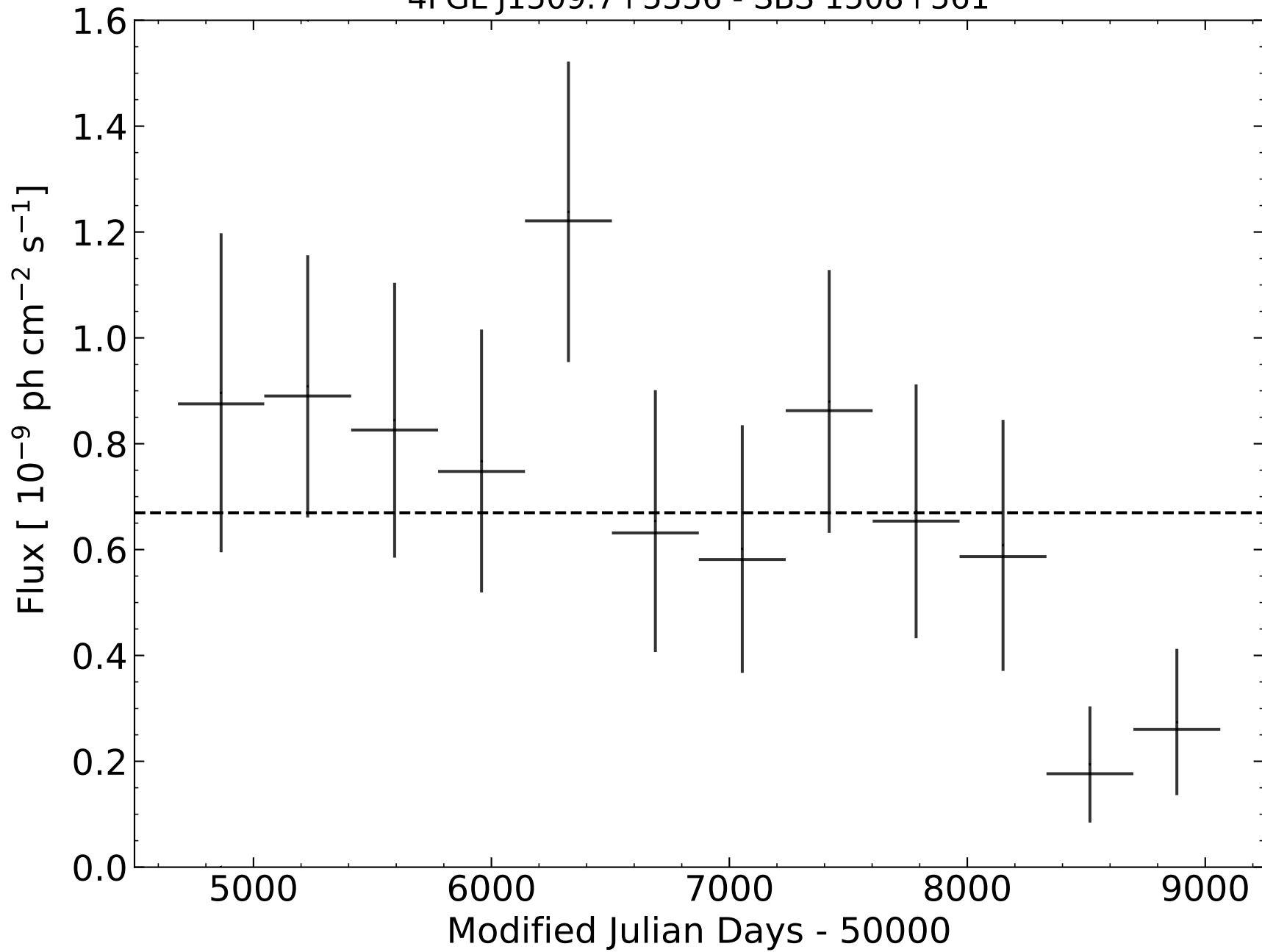
4FGL J1509.7+5556 - SBS 1508+561
