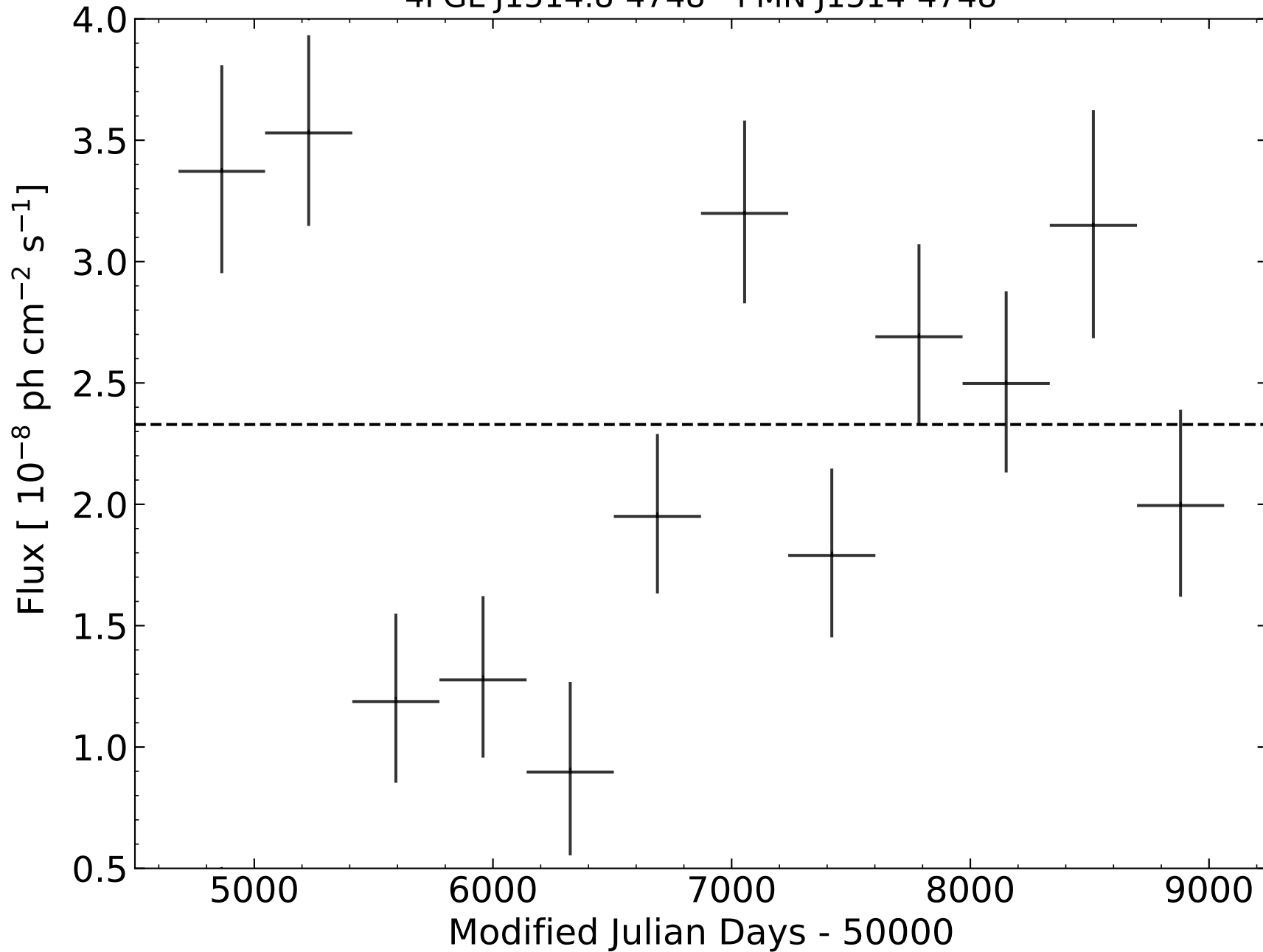
4FGL J1514.8-4748 - PMN J1514-4748
