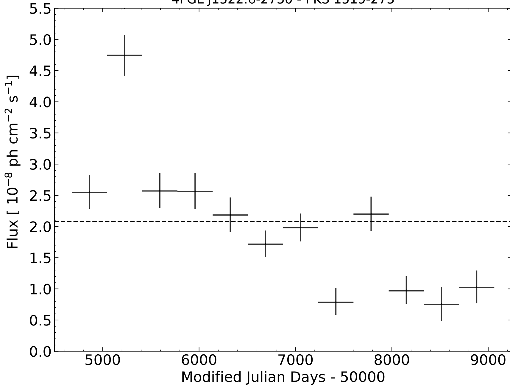
4FGL J1522.6-2730 - PKS 1519-273
