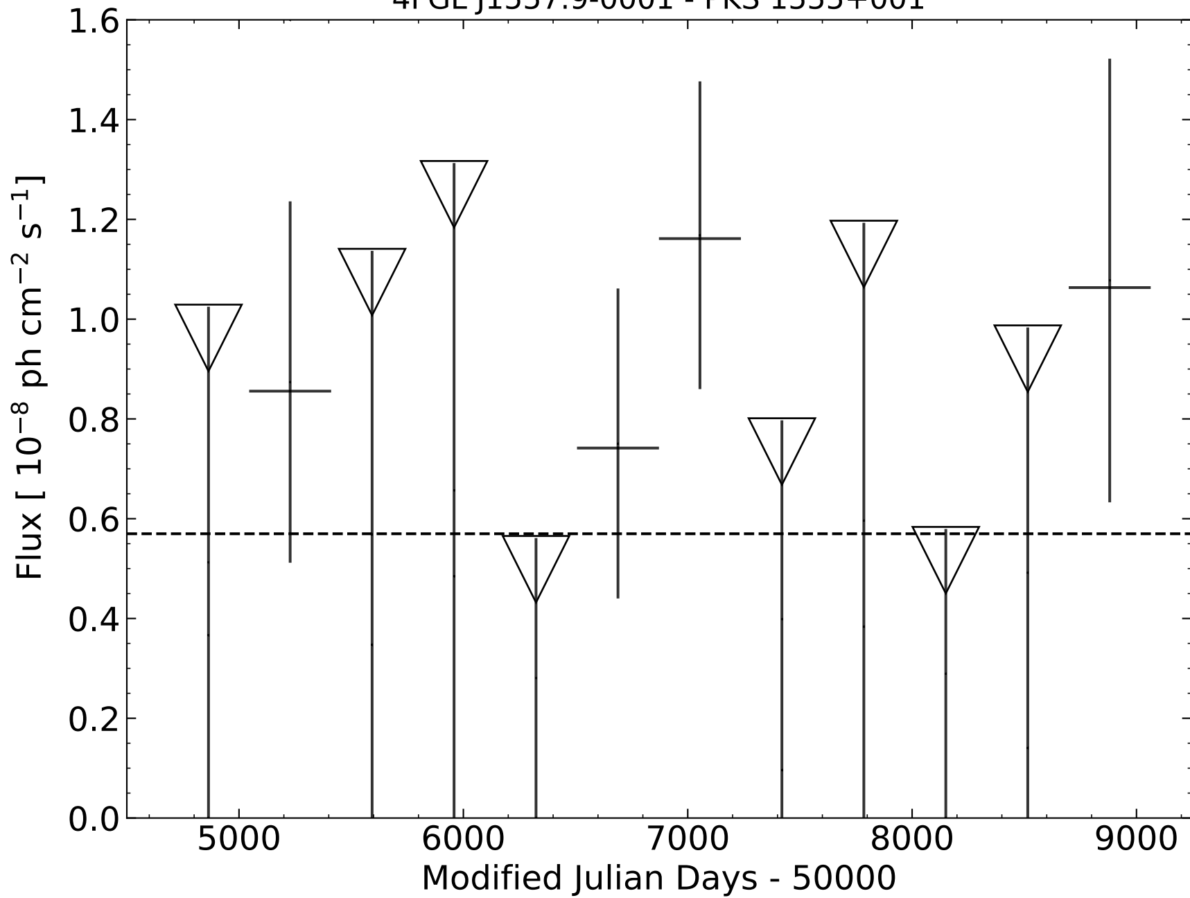
4FGL J1557.9-0001 - PKS 1555+001
