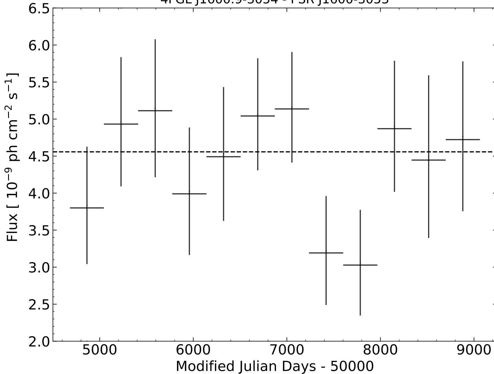
4FGL J1600.9-3054 - PSR J1600-3053
