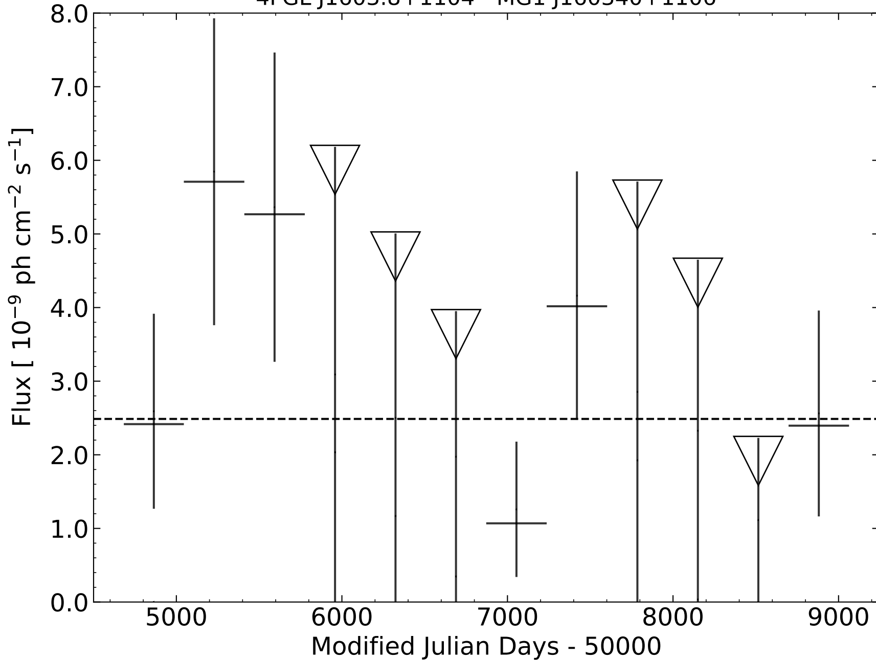
4FGL J1603.8+1104 - MG1 J160340+1106
