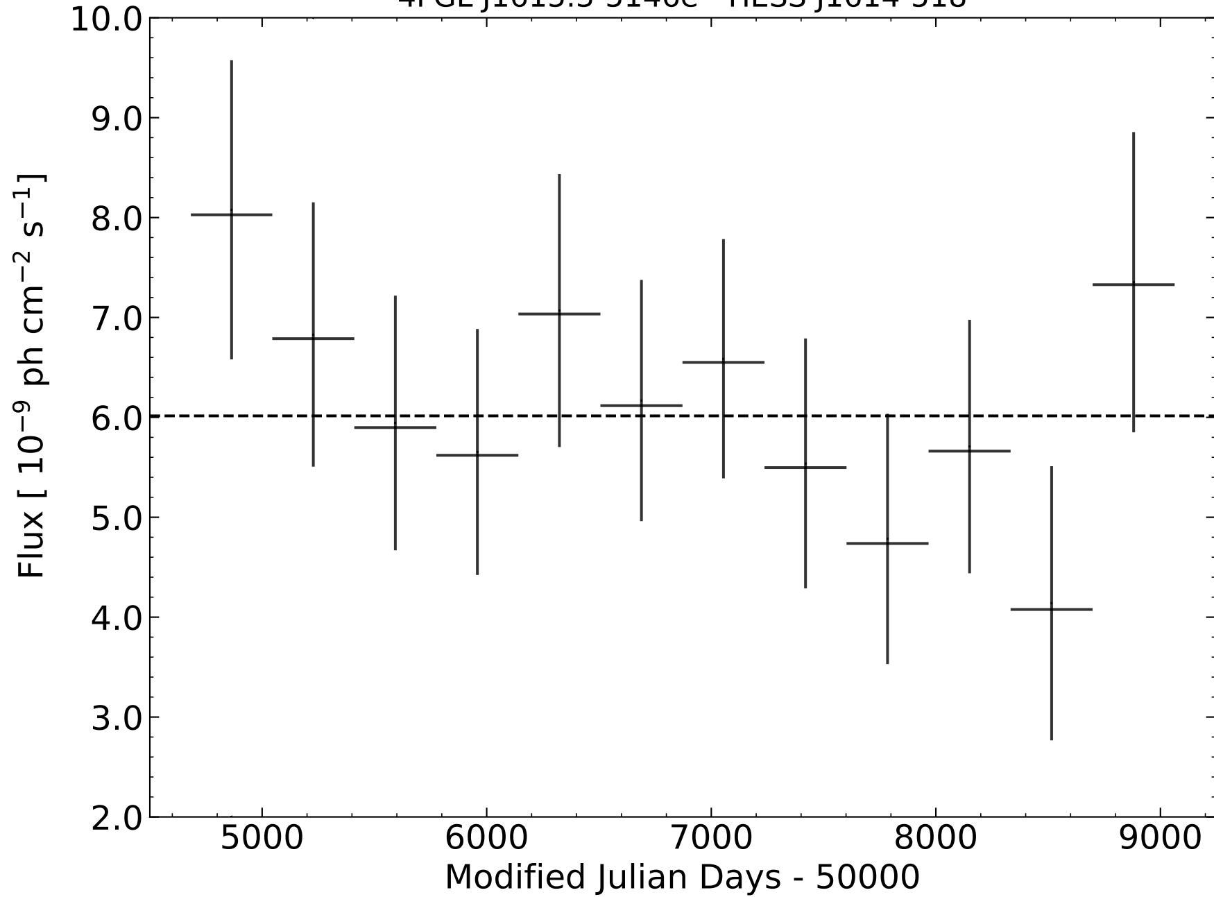
4FGL J1615.3-5146e - HESS J1614-518
