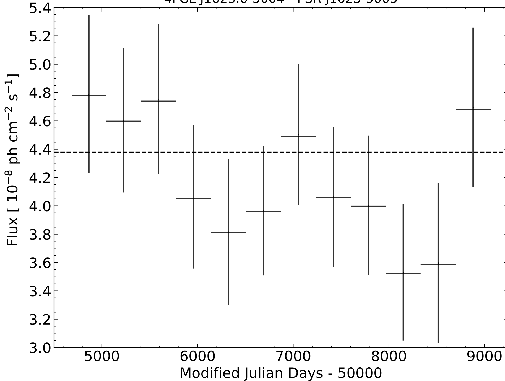
4FGL J1623.0-5004 - PSR J1623-5005
