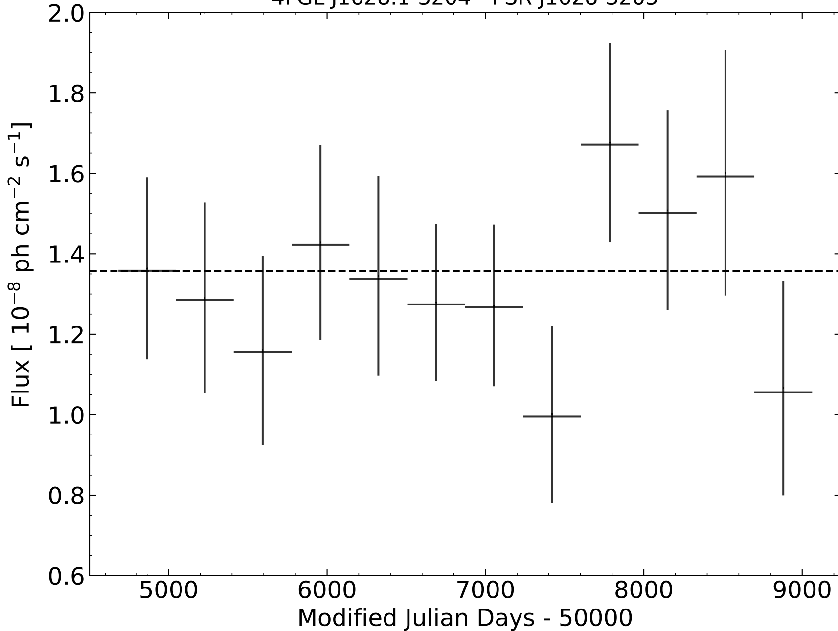
4FGL J1628.1-3204 - PSR J1628-3205
