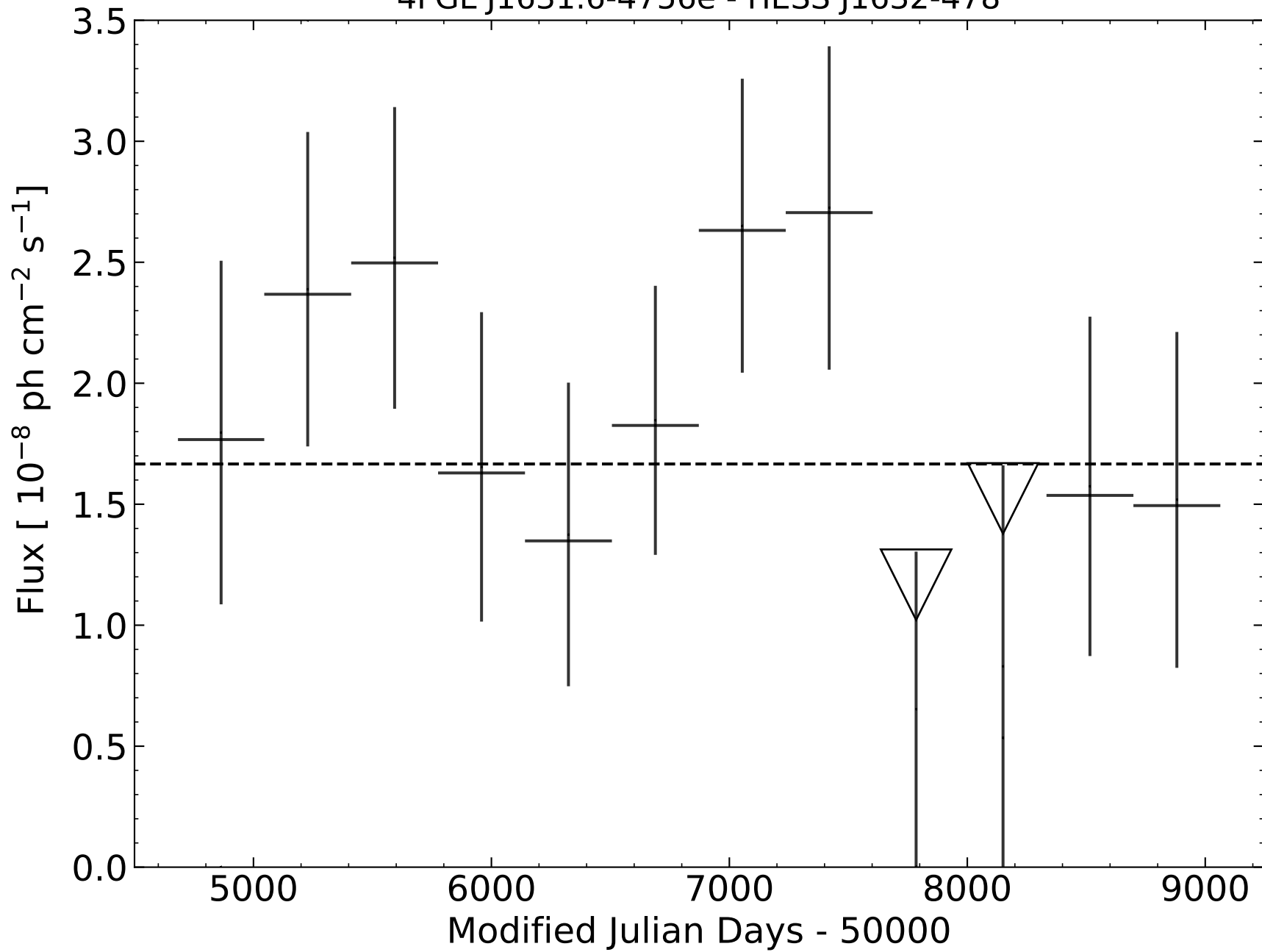
4FGL J1631.6-4756e - HESS J1632-478
