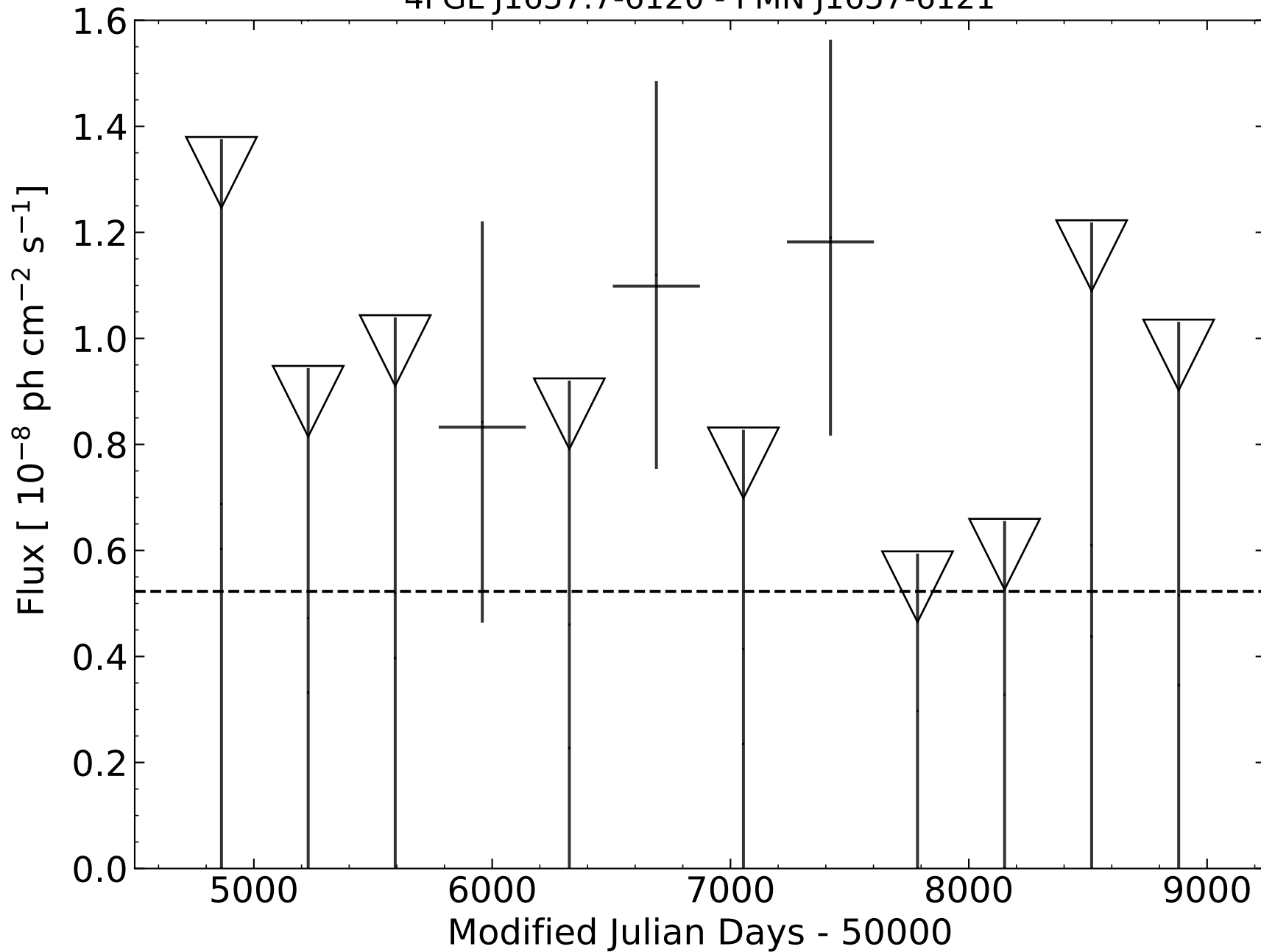
4FGL J1657.7-6120 - PMN J1657-6121
