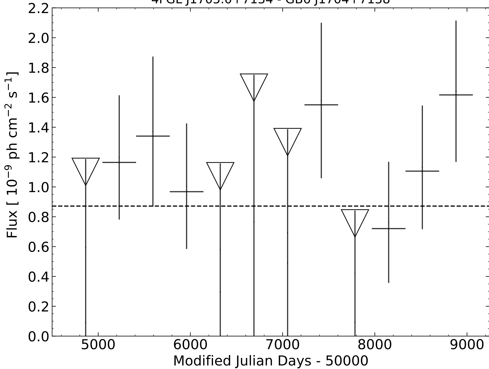
4FGL J1705.0+7134 - GB6 J1704+7138
