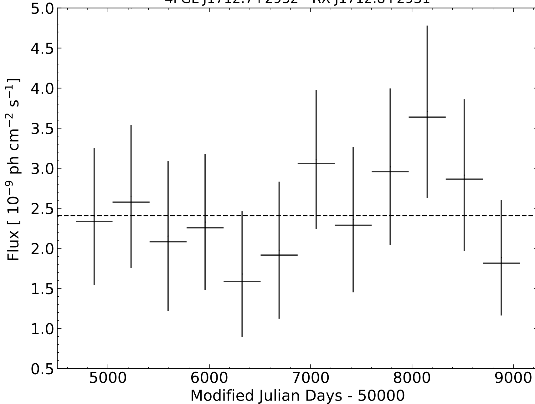
4FGL J1712.7+2932 - RX J1712.8+2931
