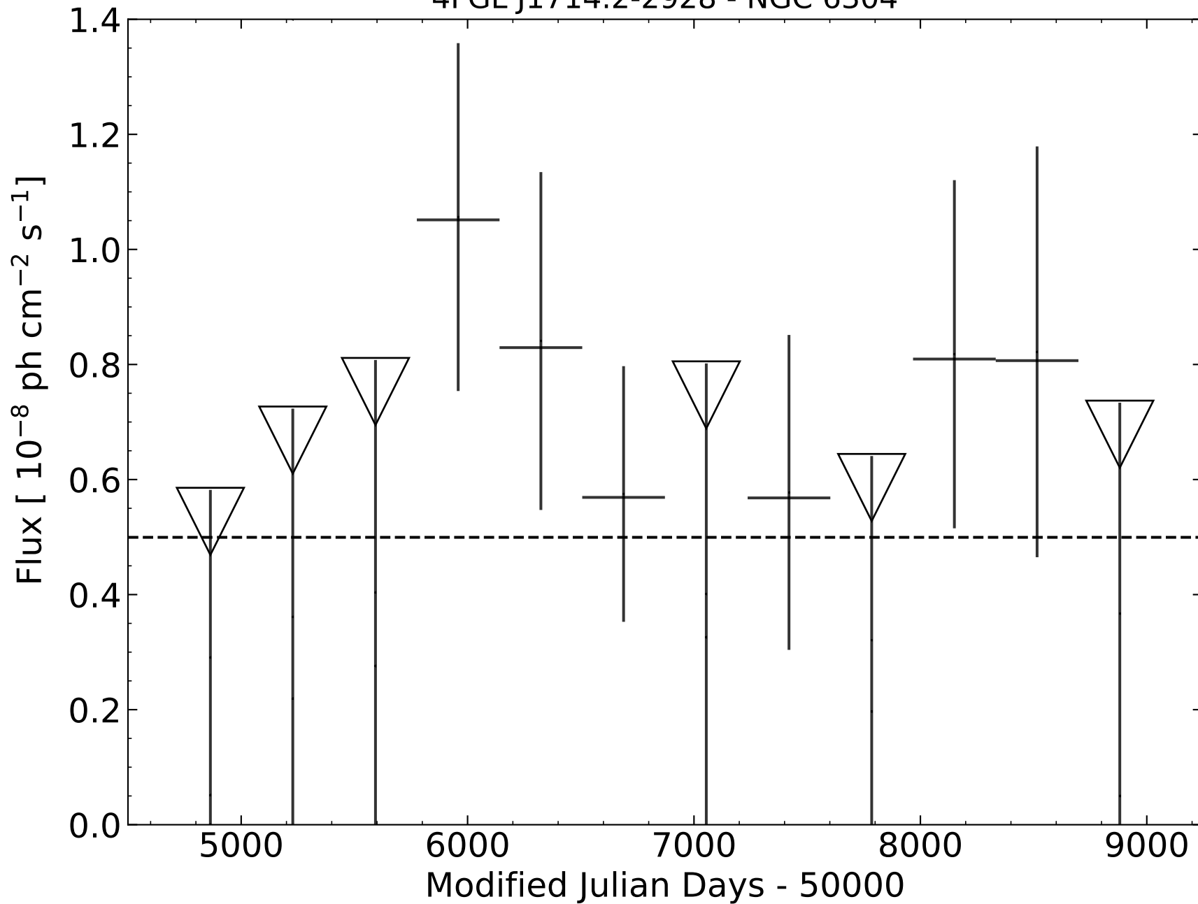
4FGL J1714.2-2928 - NGC 6304
