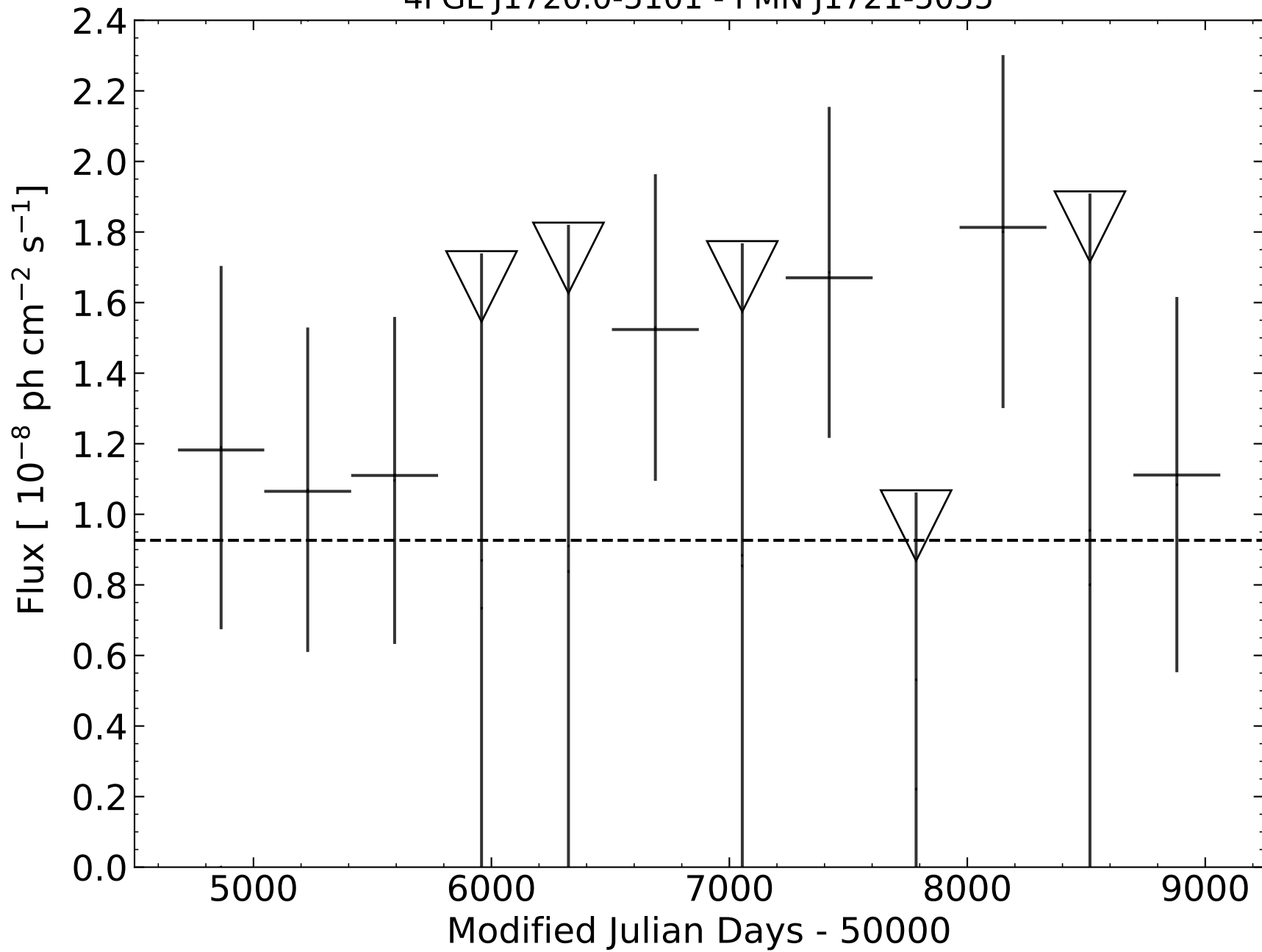
4FGL J1720.0-5101 - PMN J1721-5055
