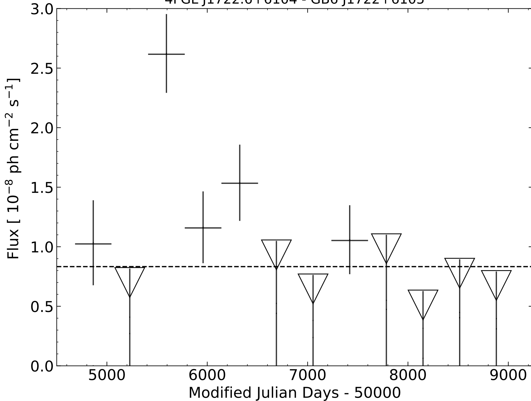
4FGL J1722.6+6104 - GB6 J1722+6105
