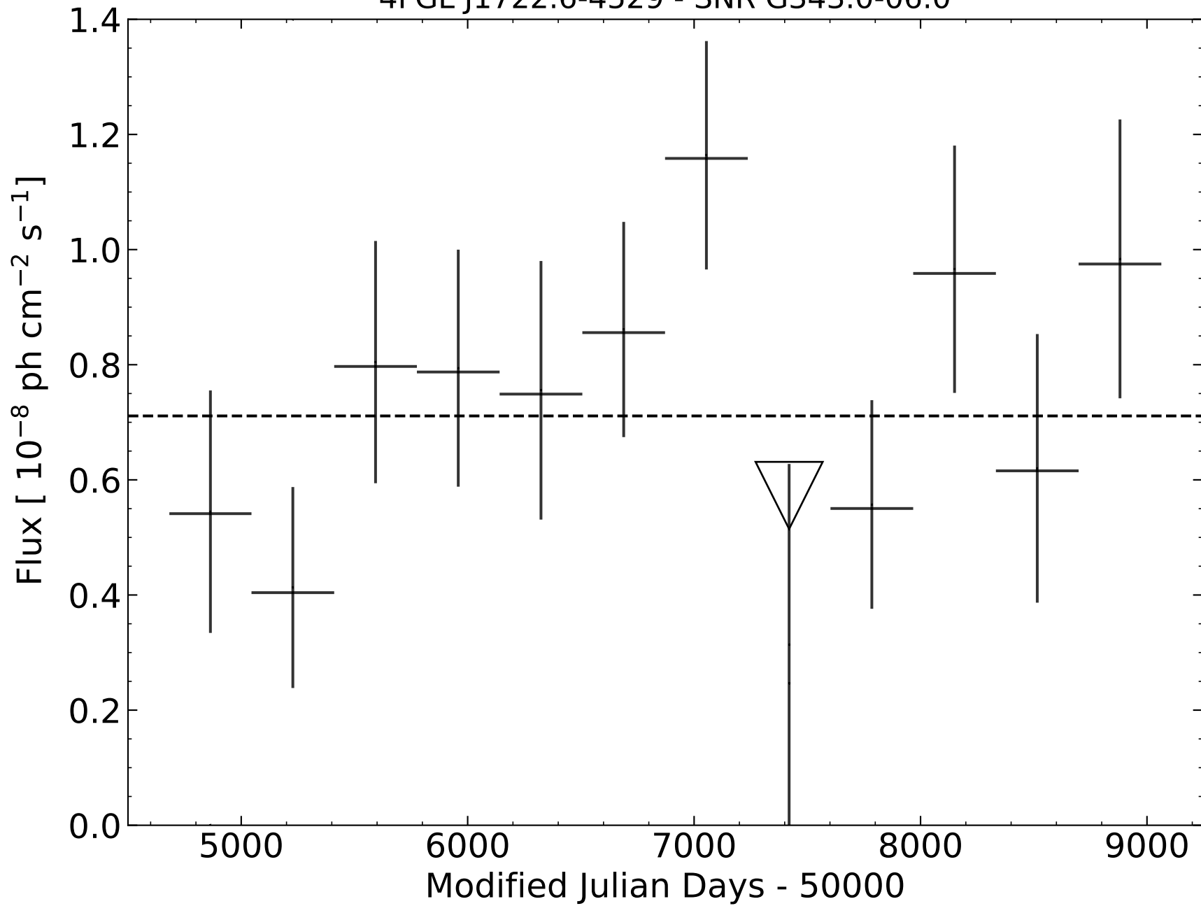
4FGL J1722.6-4529 - SNR G343.0-06.0
