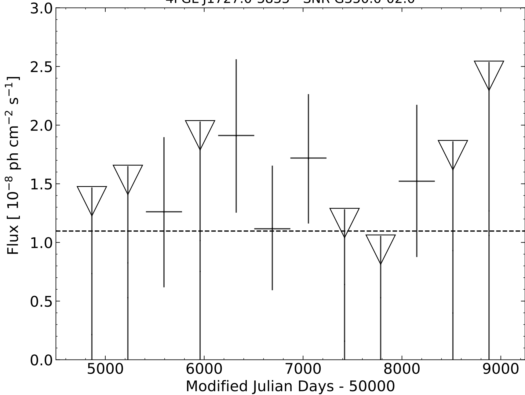
4FGL J1727.0-3835 - SNR G350.0-02.0
