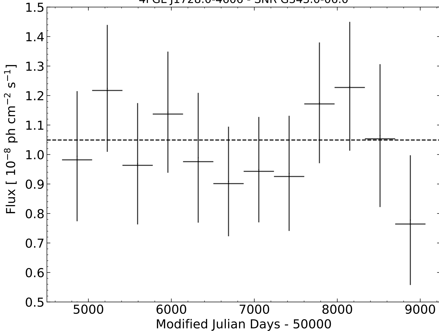
4FGL J1728.0-4606 - SNR G343.0-06.0
