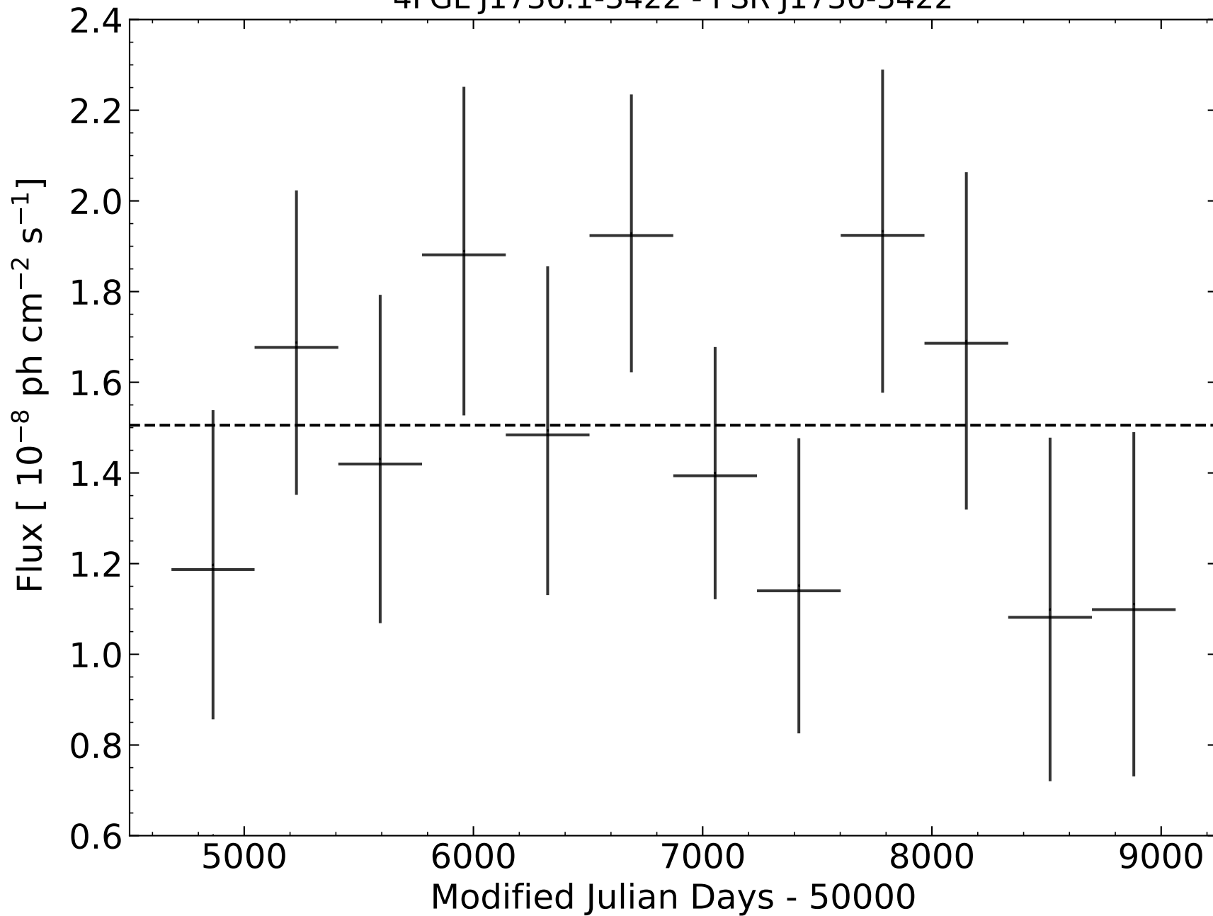
4FGL J1736.1-3422 - PSR J1736-3422
