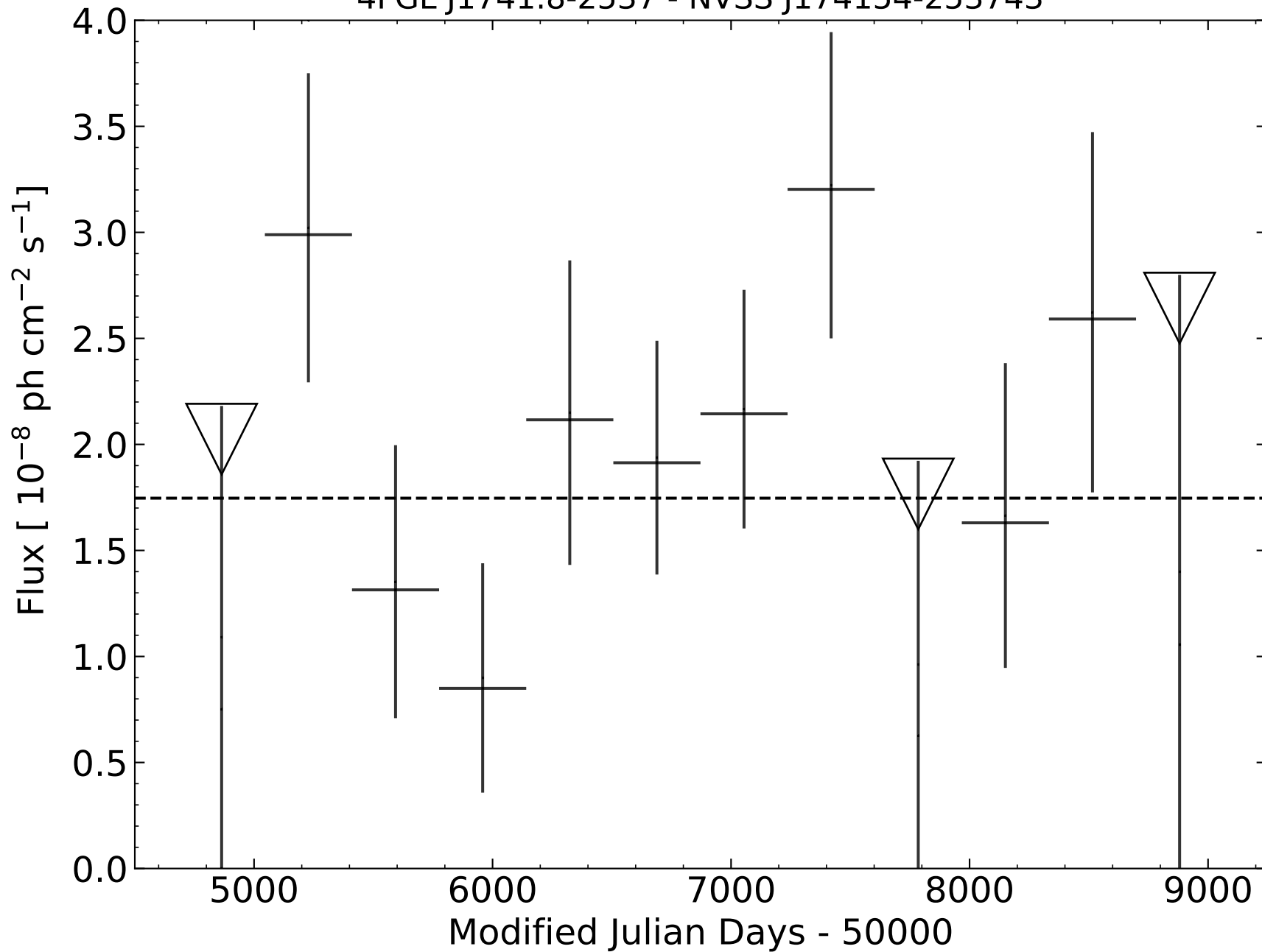
4FGL J1741.8-2537 - NVSS J174154-253743
