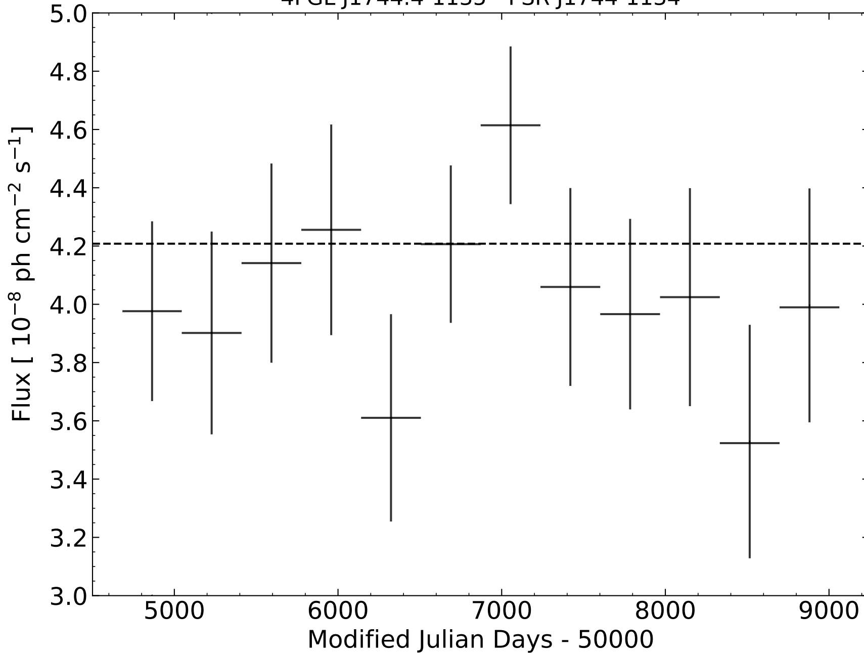
4FGL J1744.4-1135 - PSR J1744-1134
