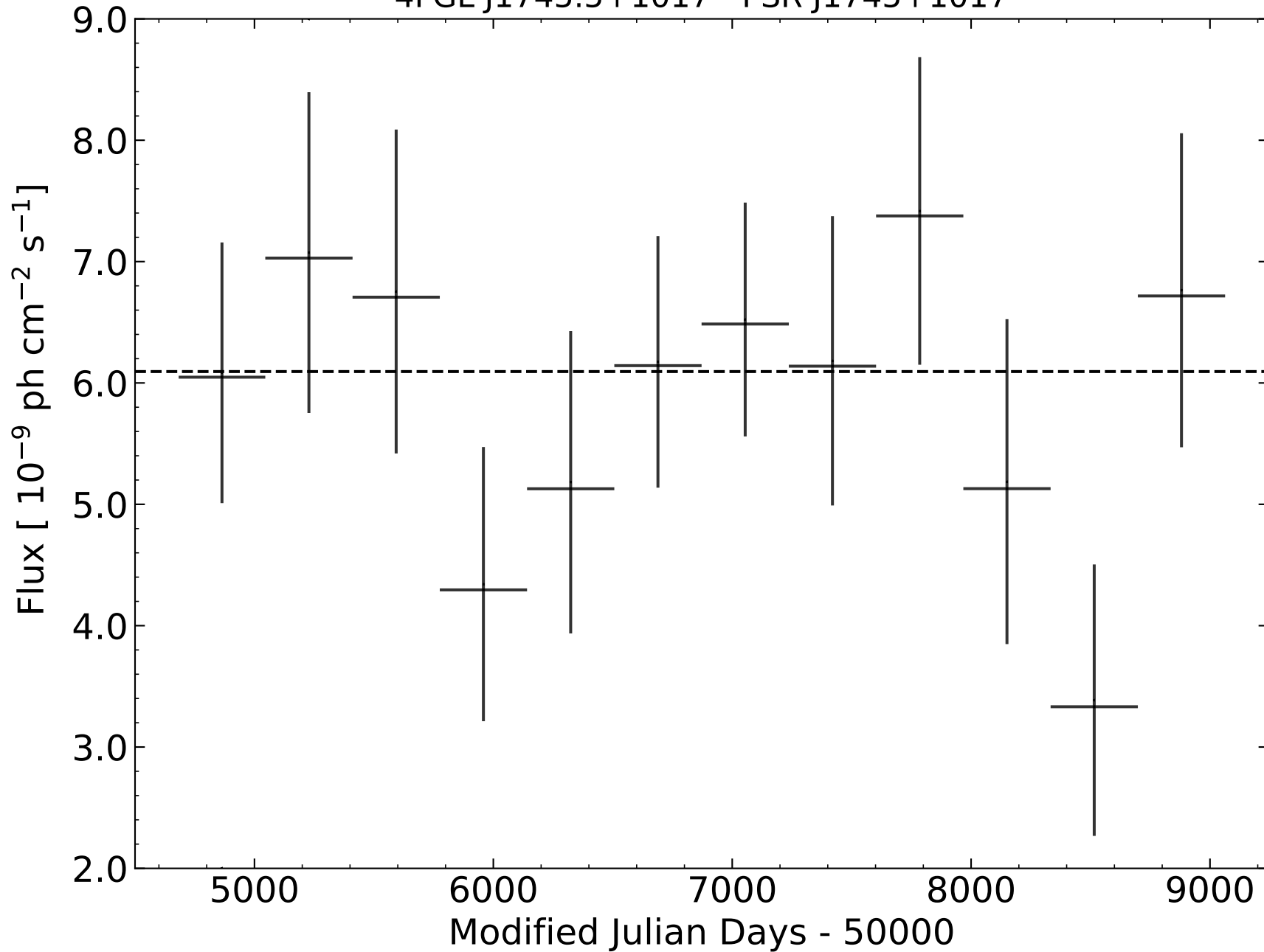
4FGL J1745.5+1017 - PSR J1745+1017
