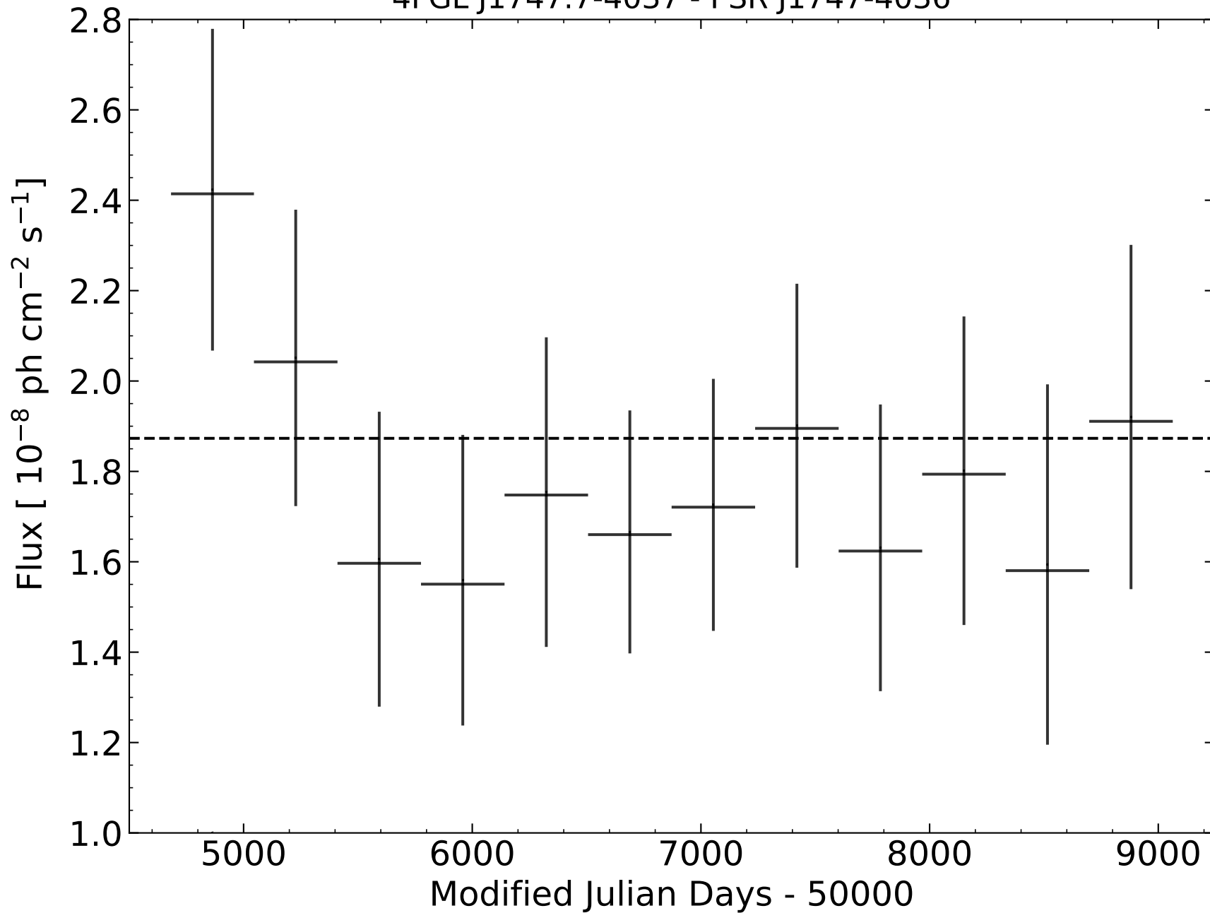
4FGL J1747.7-4037 - PSR J1747-4036
