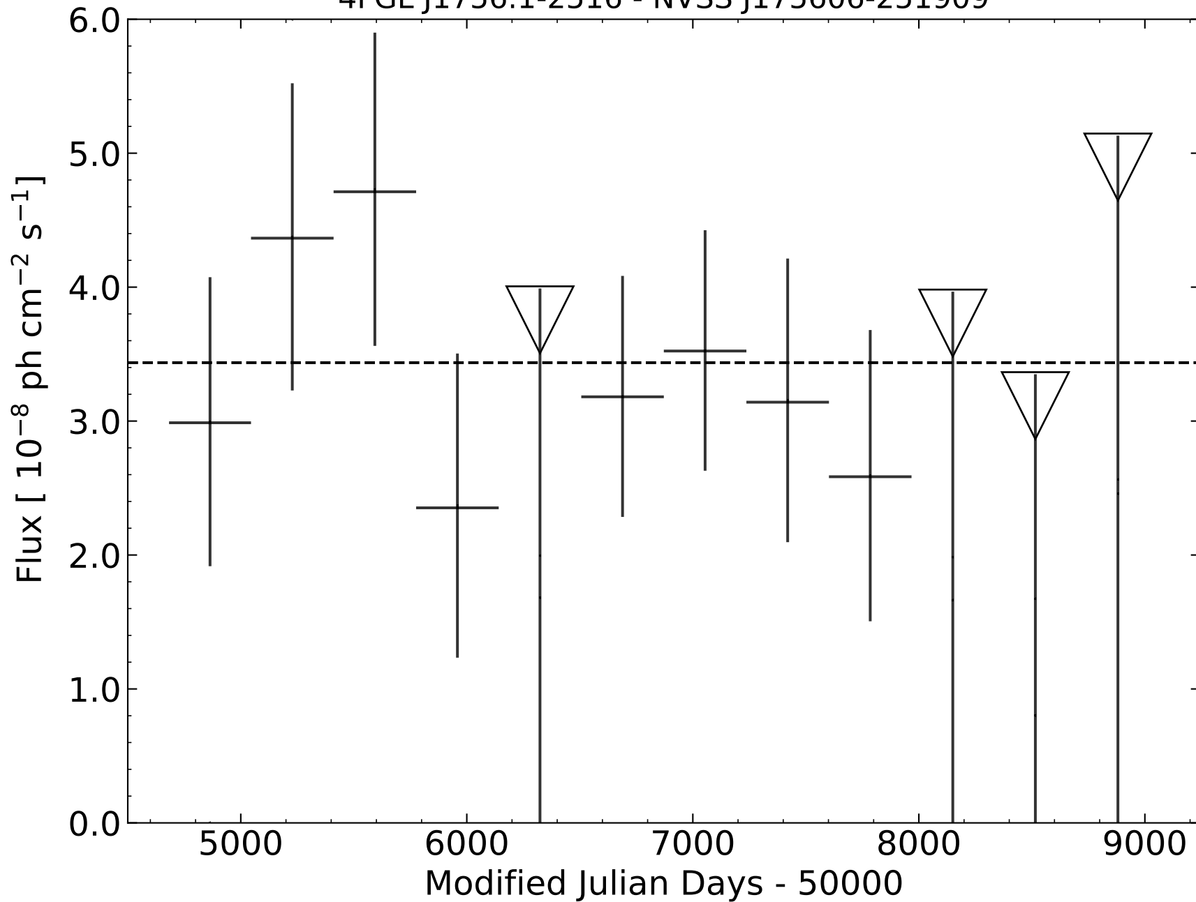
4FGL J1756.1-2516 - NVSS J175606-251909
