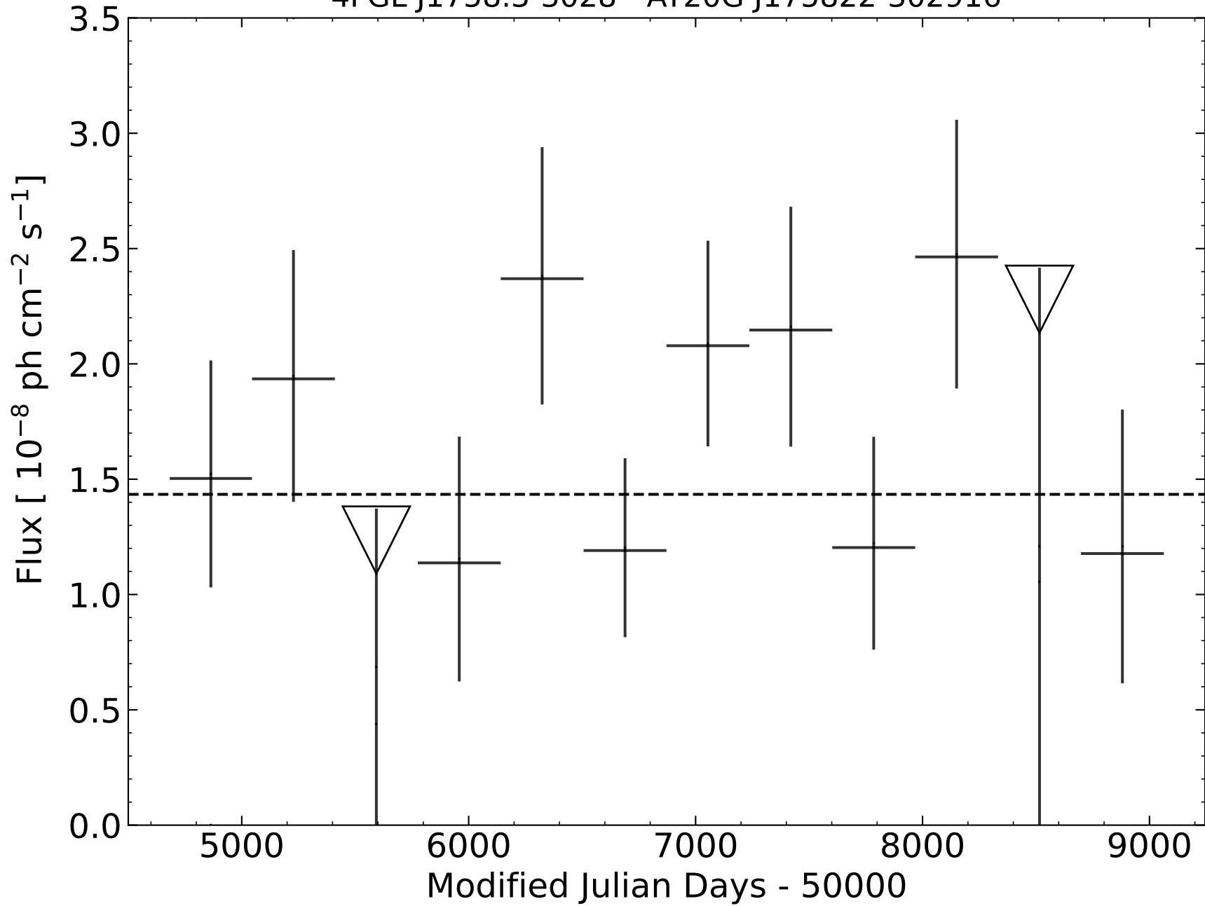
4FGL J1758.3-3028 - AT20G J175822-302916
