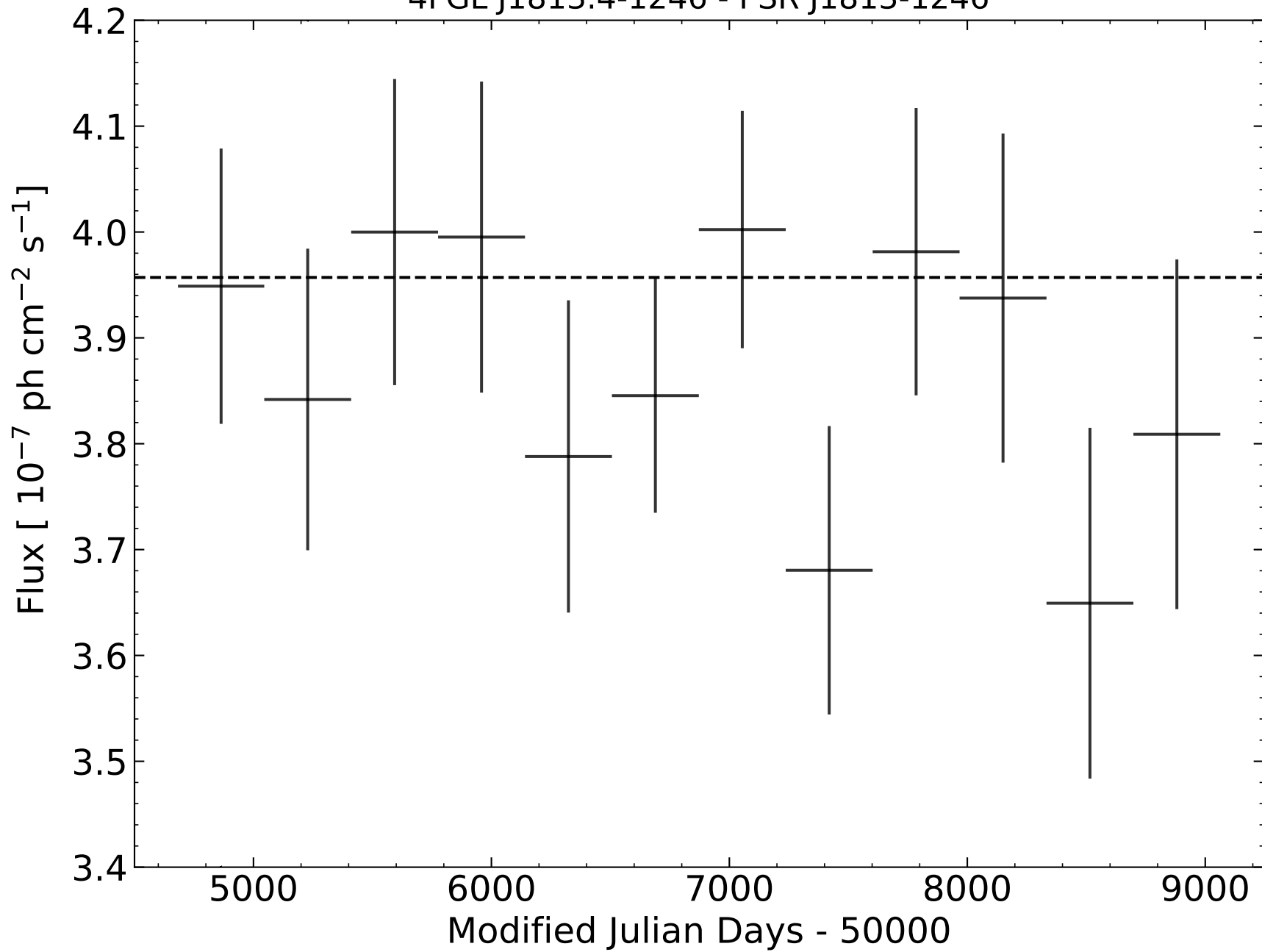
4FGL J1813.4-1246 - PSR J1813-1246
